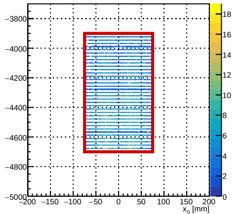
MC truth rank-0 downstream e^- origin
