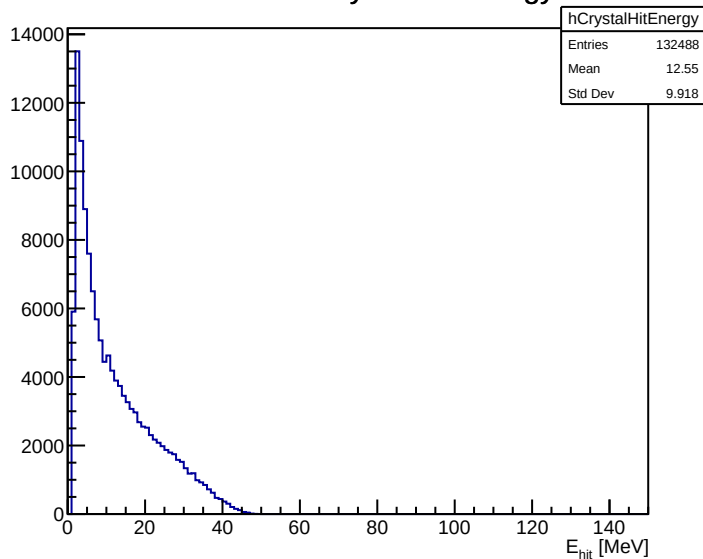
Calorimeter crystal-hit energy
