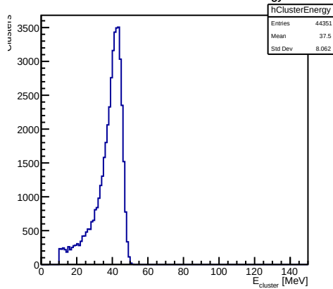
Reconstructed calorimeter cluster energy
