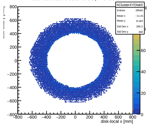
Reconstructed cluster COG, Front disk
