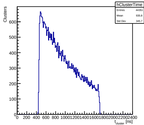
Reconstructed calorimeter cluster time
