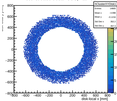
Reconstructed cluster COG, Back disk
