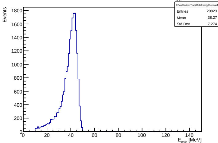
Two-track events: electron 1 calorimeter energy
