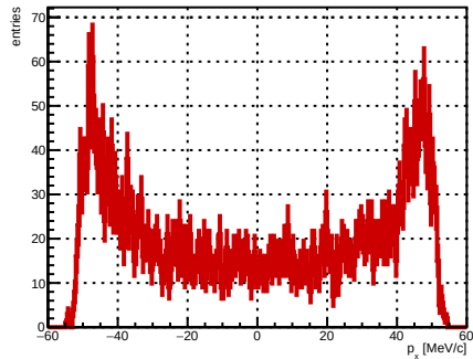
Selected track ST_Foils intersection p_x , foil index 16, N = 4494
