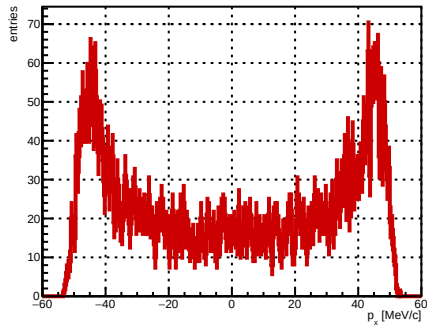
Selected track ST_Foils intersection p_x , foil index 34, N = 4972
