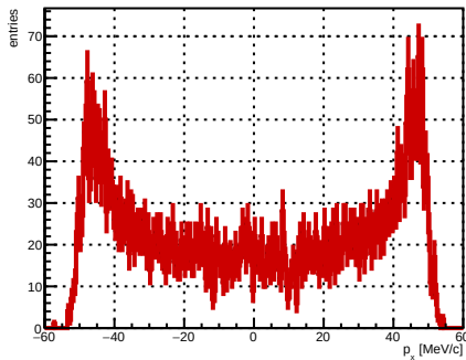
Selected track ST_Foils intersection p_x , foil index 27, N = 4945
