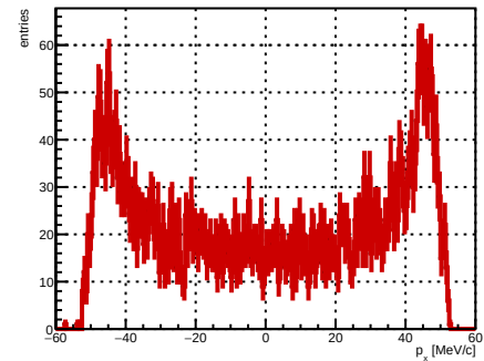
Selected track ST_Foils intersection p_x , foil index 29, N = 4850
