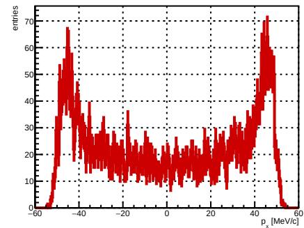
Selected track ST_Foils intersection p_x , foil index 32, N = 4920
