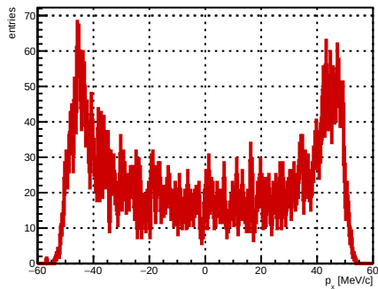
Selected track ST_Foils intersection p_x , foil index 31, N = 4961
