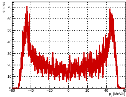
Selected track ST_Foils intersection p_x , foil index 33, N = 4938
