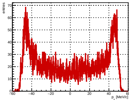
Selected track ST_Foils intersection p_x , foil index 30, N = 4938
