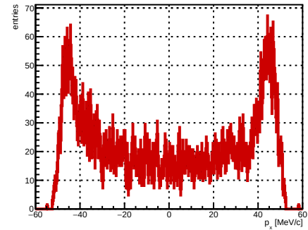
Selected track ST_Foils intersection p_x , foil index 35, N = 4836
