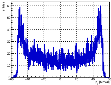
Selected track ST_Foils intersection p_y , foil index 4, N = 4128
