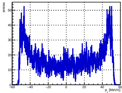
Selected track ST_Foils intersection p_y , foil index 0, N = 3700
