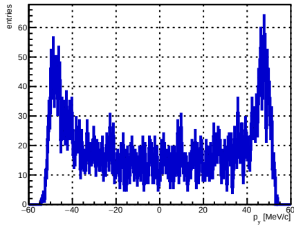
Selected track ST_Foils intersection p_y , foil index 6, N = 4116
