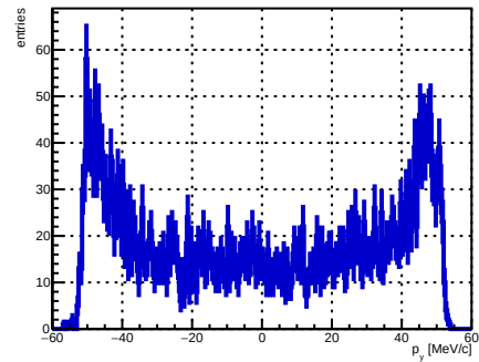
Selected track ST_Foils intersection p_y , foil index 5, N = 4105
