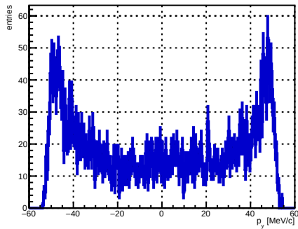
Selected track ST_Foils intersection p_y , foil index 3, N = 4056
