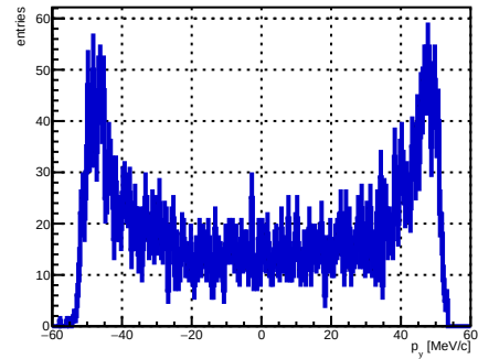
Selected track ST_Foils intersection p_y , foil index 8, N = 4245
