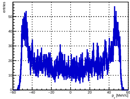
Selected track ST_Foils intersection p_y , foil index 7, N = 4164
