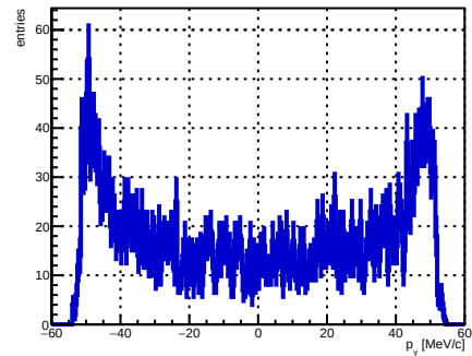
Selected track ST_Foils intersection p_y , foil index 2, N = 3881
