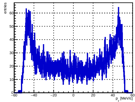
Selected track ST_Foils intersection p_y , foil index 26, N = 5042
