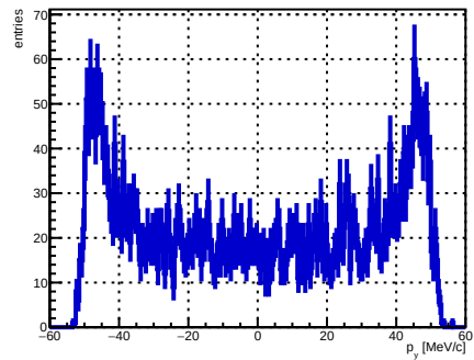
Selected track ST_Foils intersection p_y , foil index 23, N = 4878
