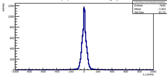
TEST: minimum- |\Delta t| vertex minus truth origin y difference
