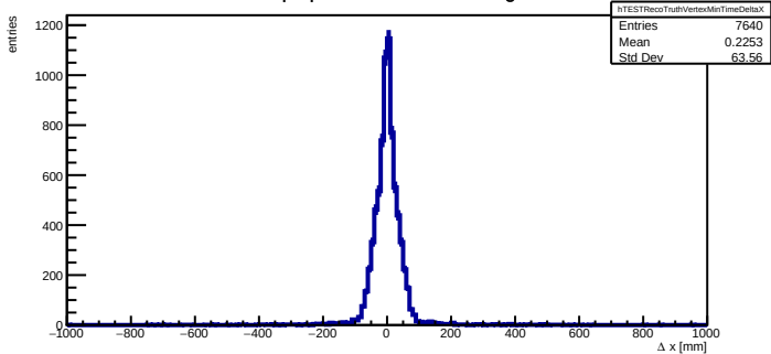
TEST: minimum- |\Delta t| vertex minus truth origin x difference
