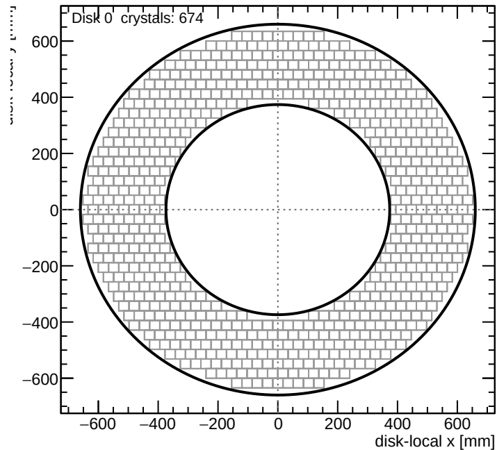
Calorimeter disk 0
