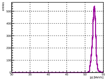
Selected track ST_Foils intersection |p|, foil index 7, N = 3291
