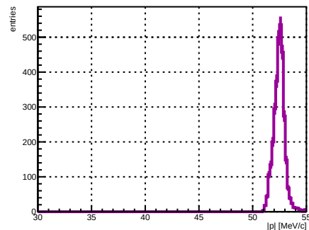
Selected track ST_Foils intersection |p|, foil index 5, N = 3277
