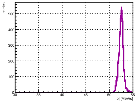
Selected track ST_Foils intersection |p|, foil index 4, N = 3283
