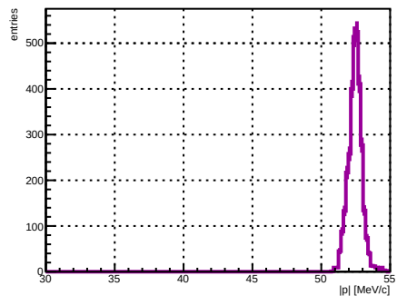
Selected track ST_Foils intersection |p|, foil index 6, N = 3193
