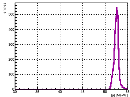
Selected track ST_Foils intersection |p|, foil index 3, N = 3173
