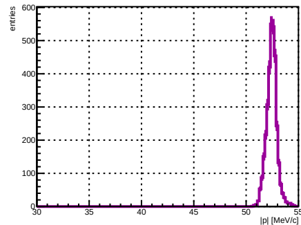
Selected track ST_Foils intersection |p|, foil index 8, N = 3370
