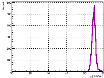
Selected track ST_Foils intersection |p|, foil index 13, N = 3563
