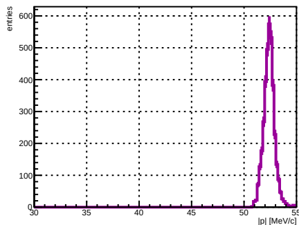
Selected track ST_Foils intersection |p|, foil index 16, N = 3644
