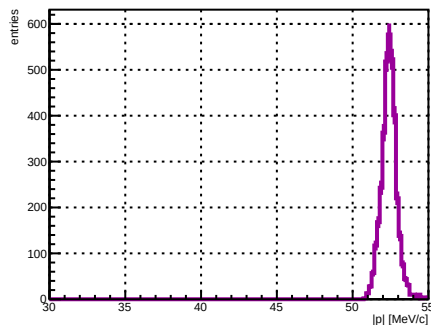
Selected track ST_Foils intersection |p|, foil index 15, N = 3576
