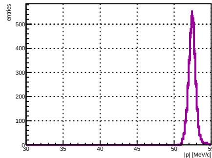
Selected track ST_Foils intersection |p|, foil index 14, N = 3580
