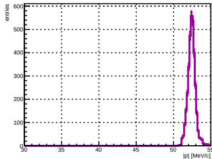
Selected track ST_Foils intersection |p|, foil index 12, N = 3507
