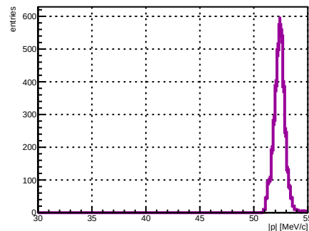
Selected track ST_Foils intersection |p|, foil index 17, N = 3678
