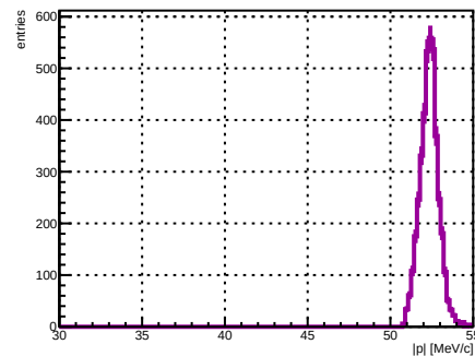
Selected track ST_Foils intersection |p|, foil index 26, N = 4058
