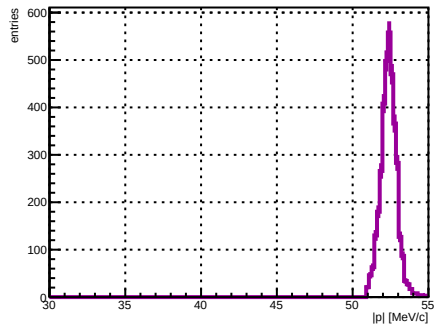
Selected track ST_Foils intersection |p|, foil index 21, N = 3895
