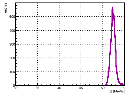
Selected track ST_Foils intersection |p|, foil index 23, N = 3848
