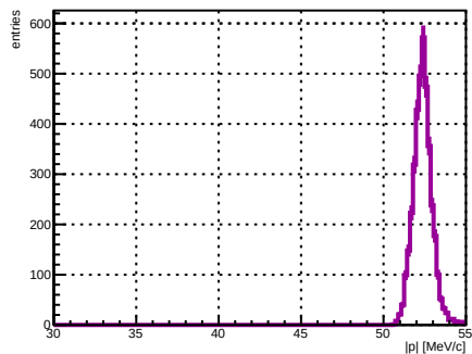
Selected track ST_Foils intersection |p|, foil index 24, N = 3868
