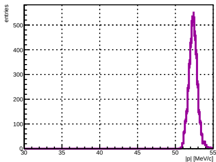
Selected track ST_Foils intersection |p|, foil index 25, N = 3926
