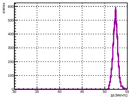
Selected track ST_Foils intersection |p|, foil index 22, N = 3845
