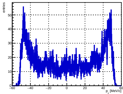
Selected track ST_Foils intersection p_y , foil index 22, N = 3845
