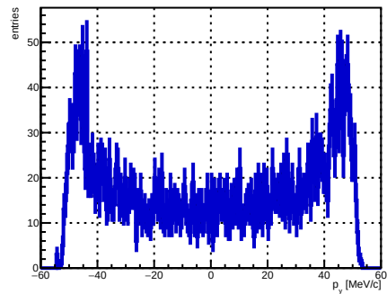
Selected track ST_Foils intersection p_y , foil index 23, N = 3848
