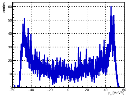
Selected track ST_Foils intersection p_y , foil index 18, N = 3624
