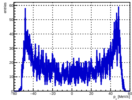
Selected track ST_Foils intersection p_y , foil index 20, N = 3782
