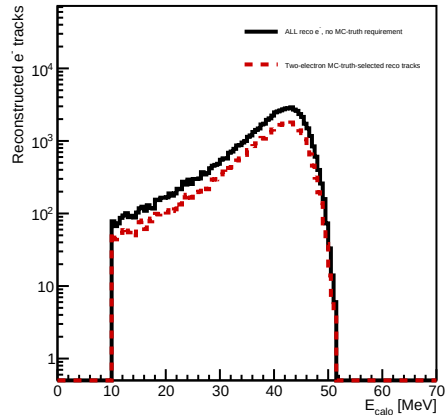
Track-associated calorimeter energy: ALL vs two-electron MC truth log y
