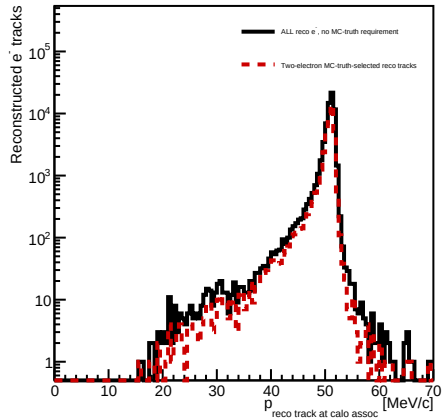
Reconstructed track momentum at track-calo association: ALL vs two-electron MC truth log y
