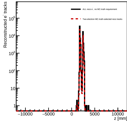
Track-calo POCA z: ALL vs two-electron MC truth log y
