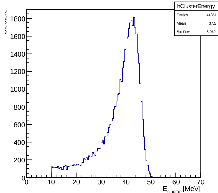
Reconstructed calorimeter cluster energy
