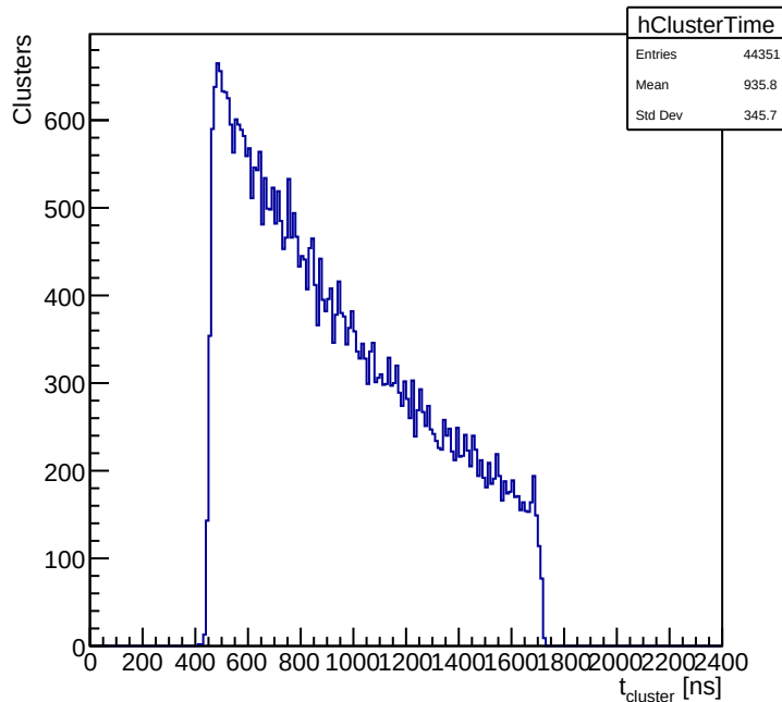
Reconstructed calorimeter cluster time
