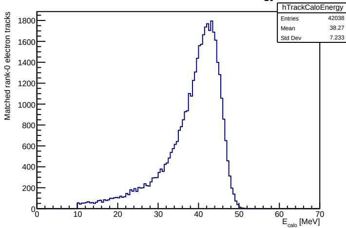
Track-associated calorimeter energy
