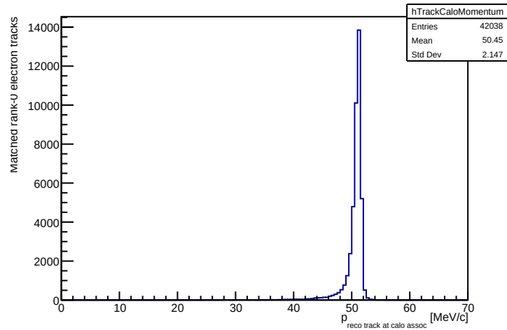
Reconstructed track momentum at track-calorimeter association
