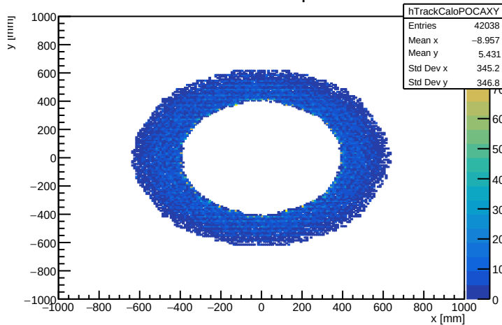
Track-calorimeter POCA position
