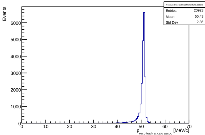
Two-track events: electron 1 reconstructed track momentum at track-calo association
