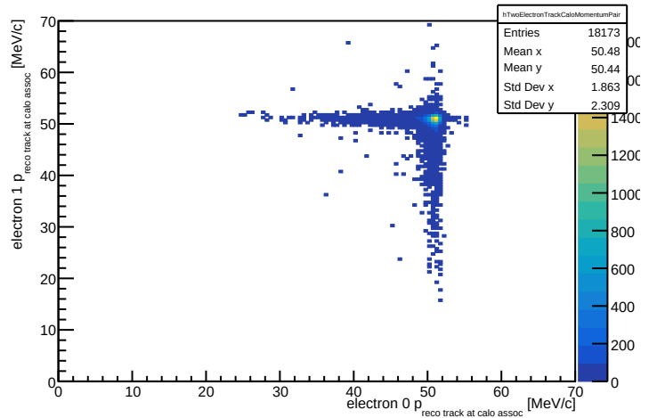
Two-track events: reconstructed track momentum pair at track-calo association
