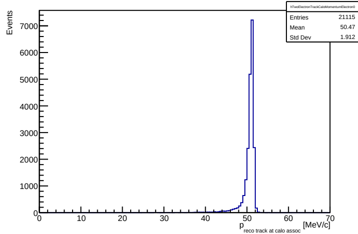
Two-track events: electron 0 reconstructed track momentum at track-calo association
