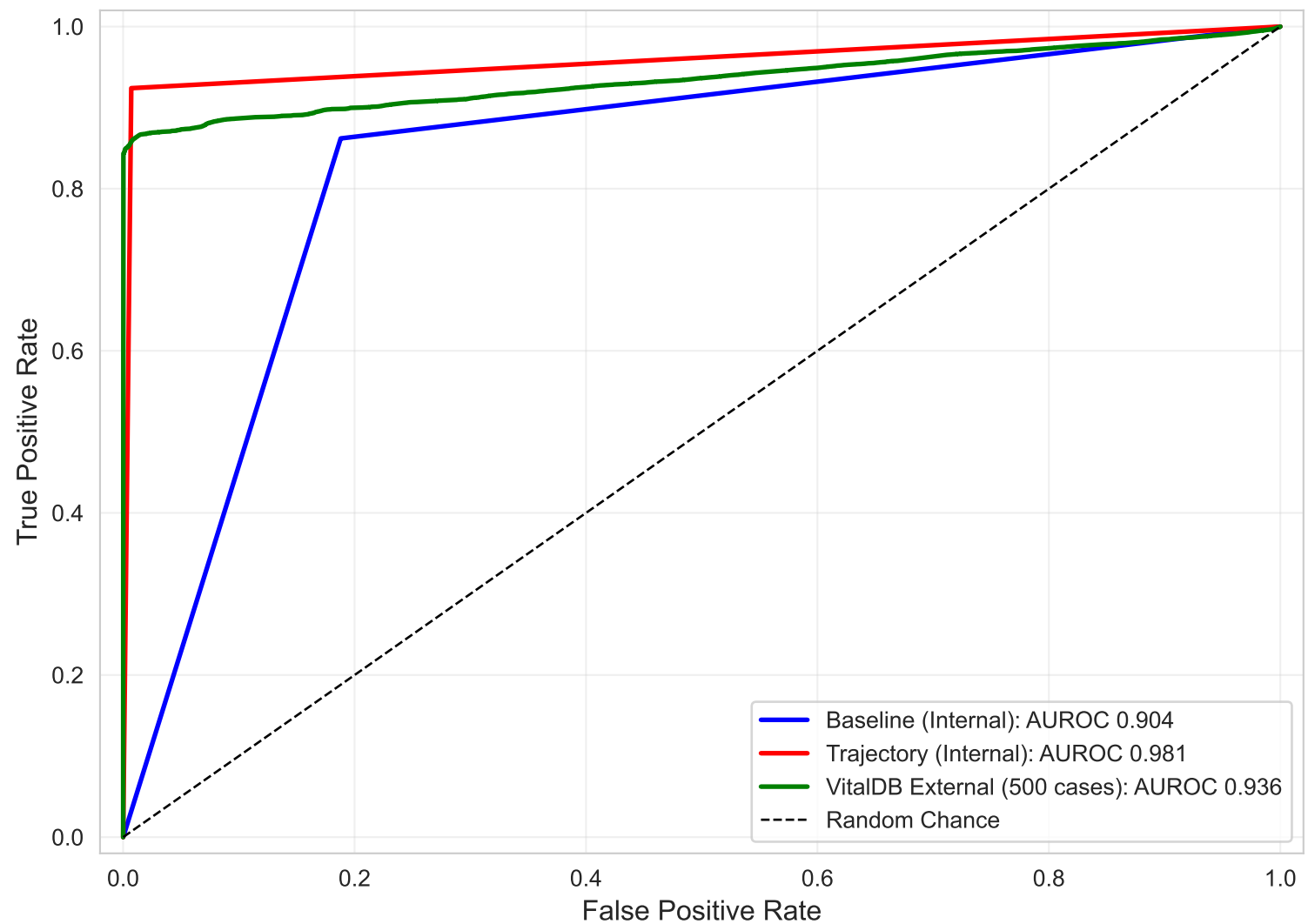
ROC Curves for Pressure Escalation Prediction
