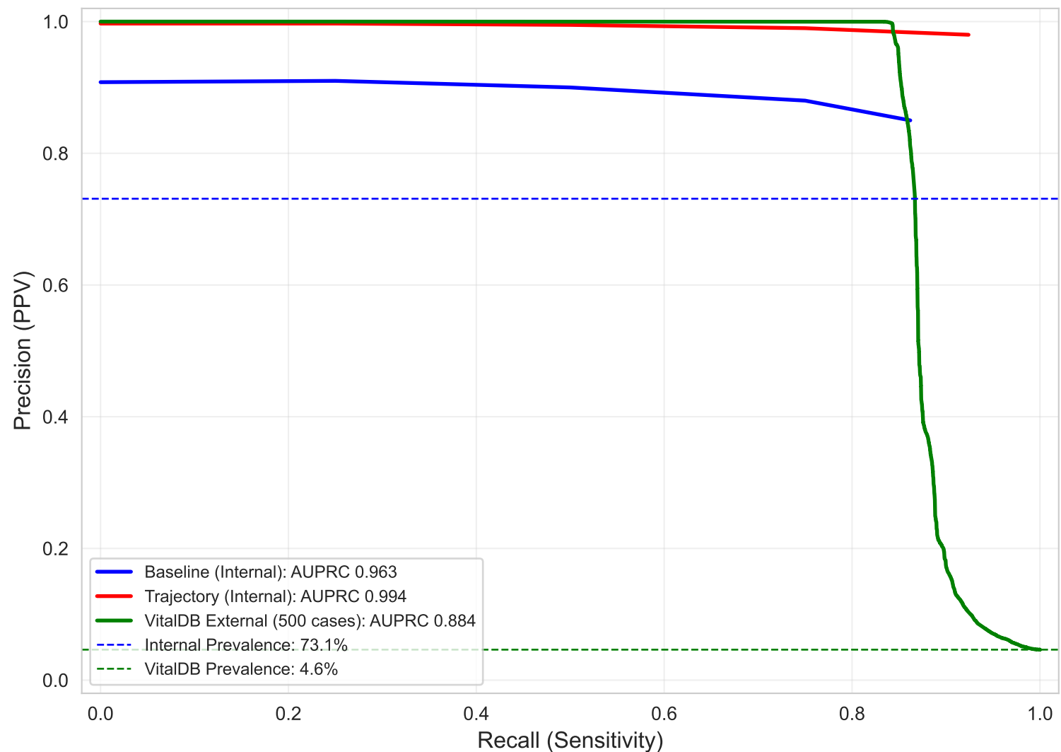
Precision-Recall Curves
