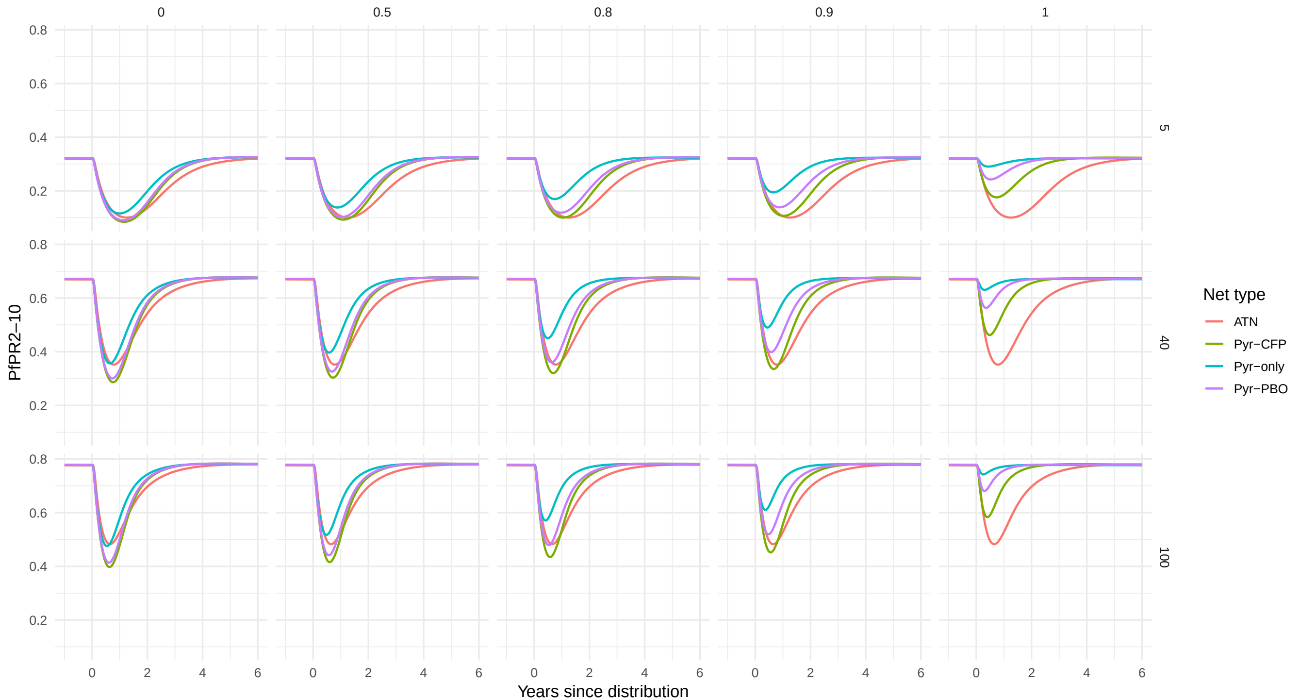
Pyrethroid resistance (columns) vs baseline EIR (rows)
