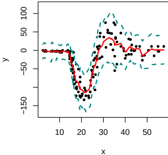
Heteroskedastic BART
