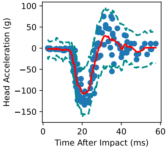
Heteroskedastic BART
