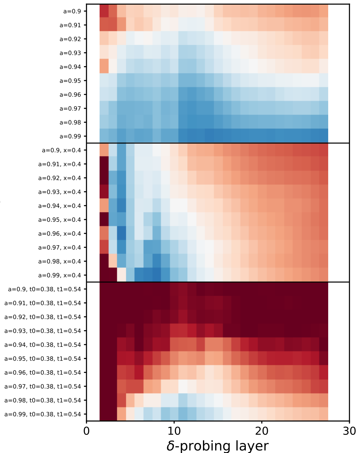
Original \delta -belief coordinate after \delta steering
