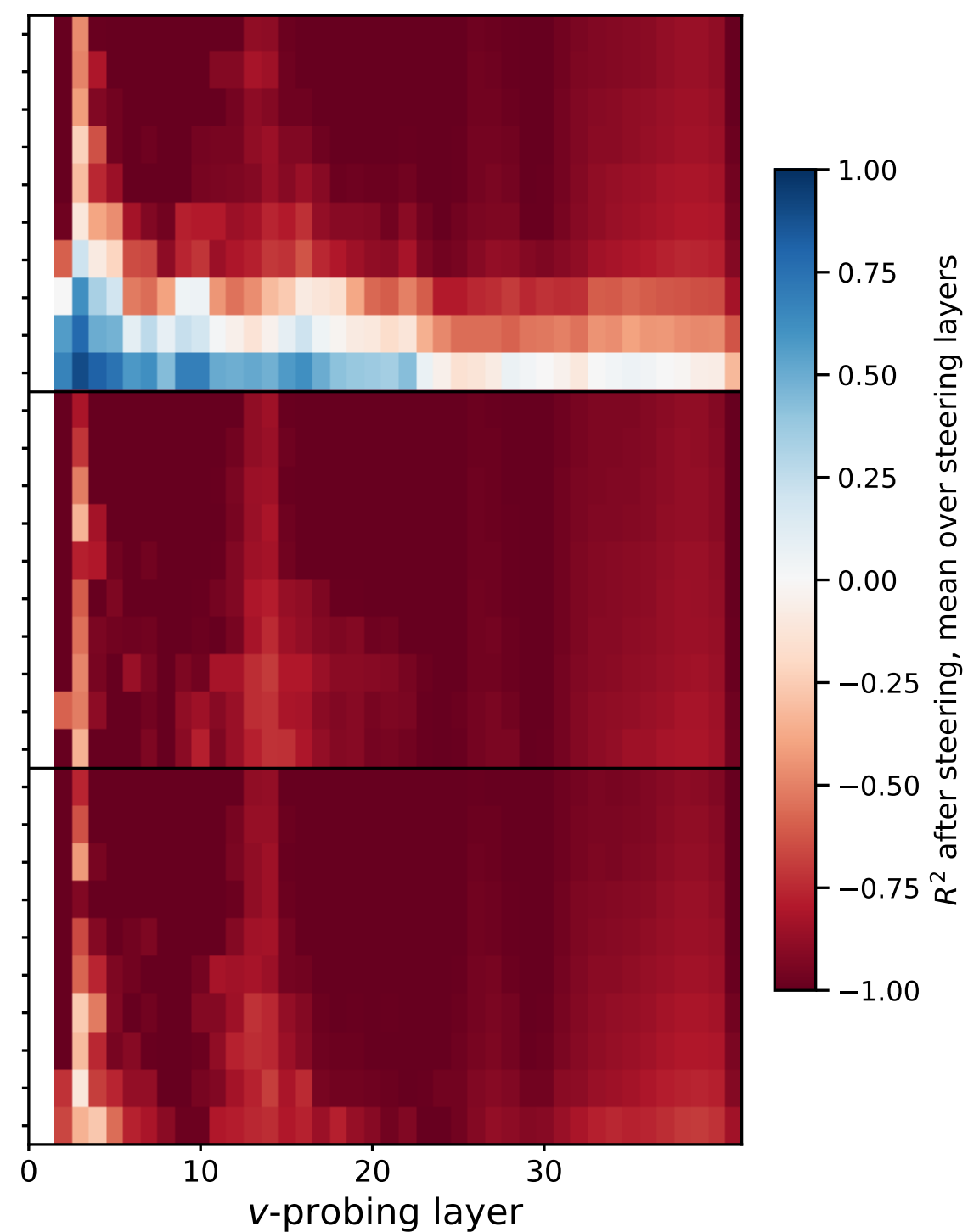
Target random component after random steering
