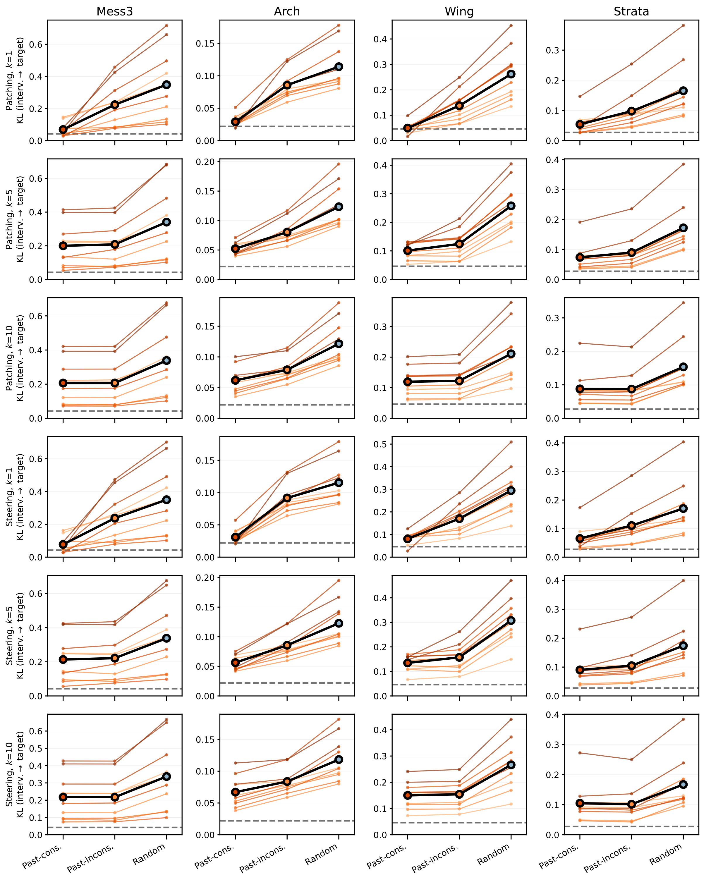
Gemma 4 E2B (lower KL: prediction closer to injected target)
