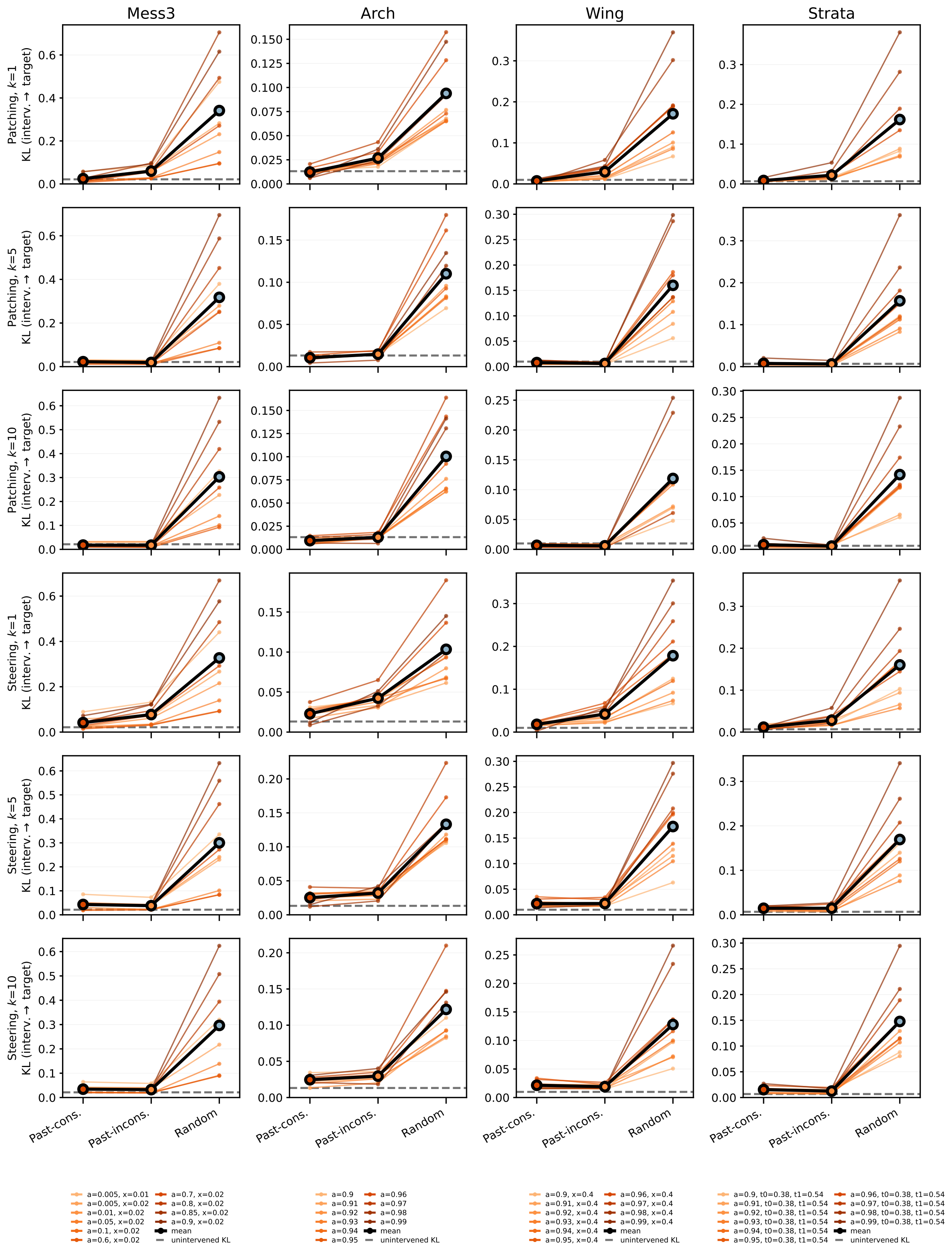
Llama 3.1 8B (lower KL: prediction closer to injected target)
