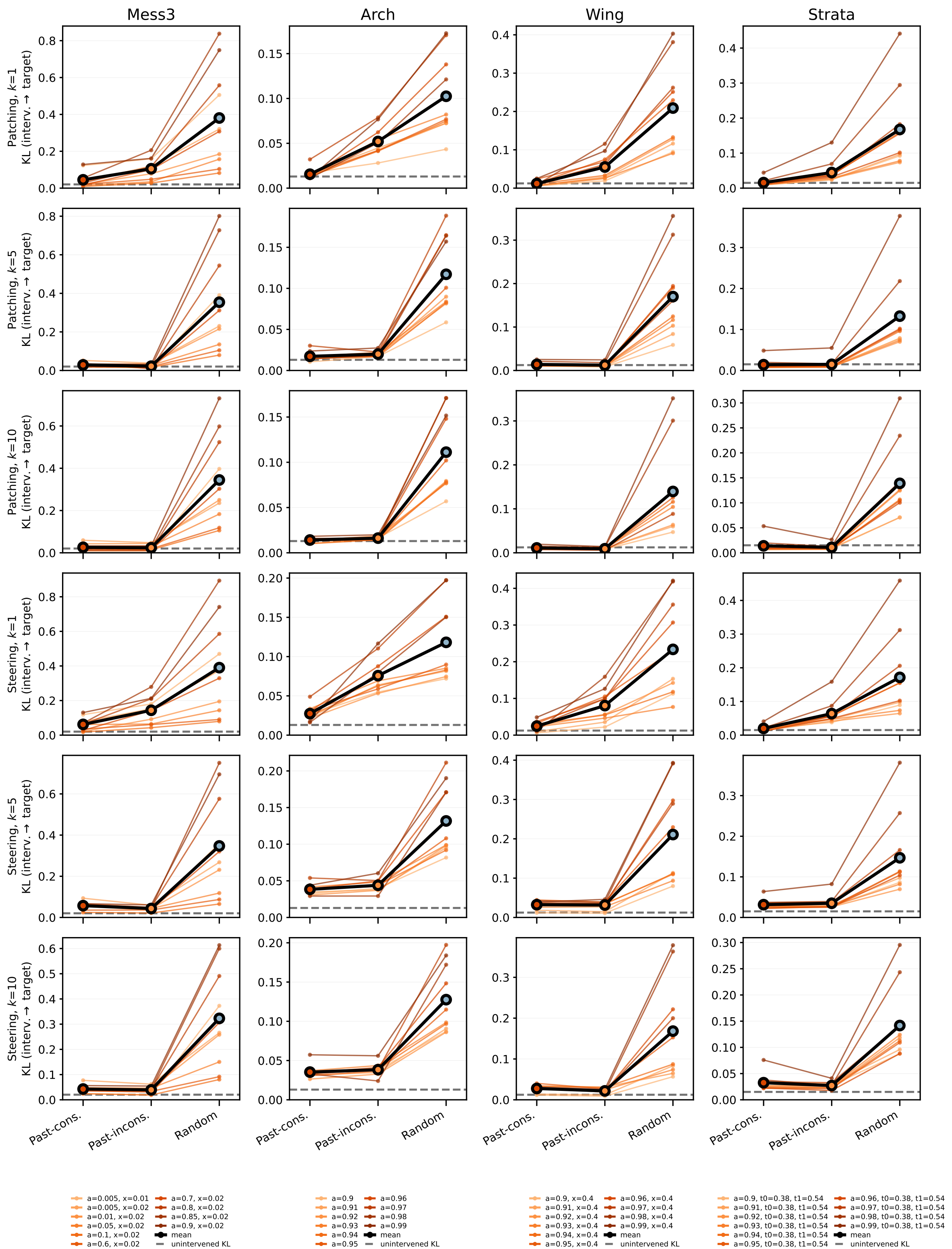
Qwen 3.5 4B (lower KL: prediction closer to injected target)
