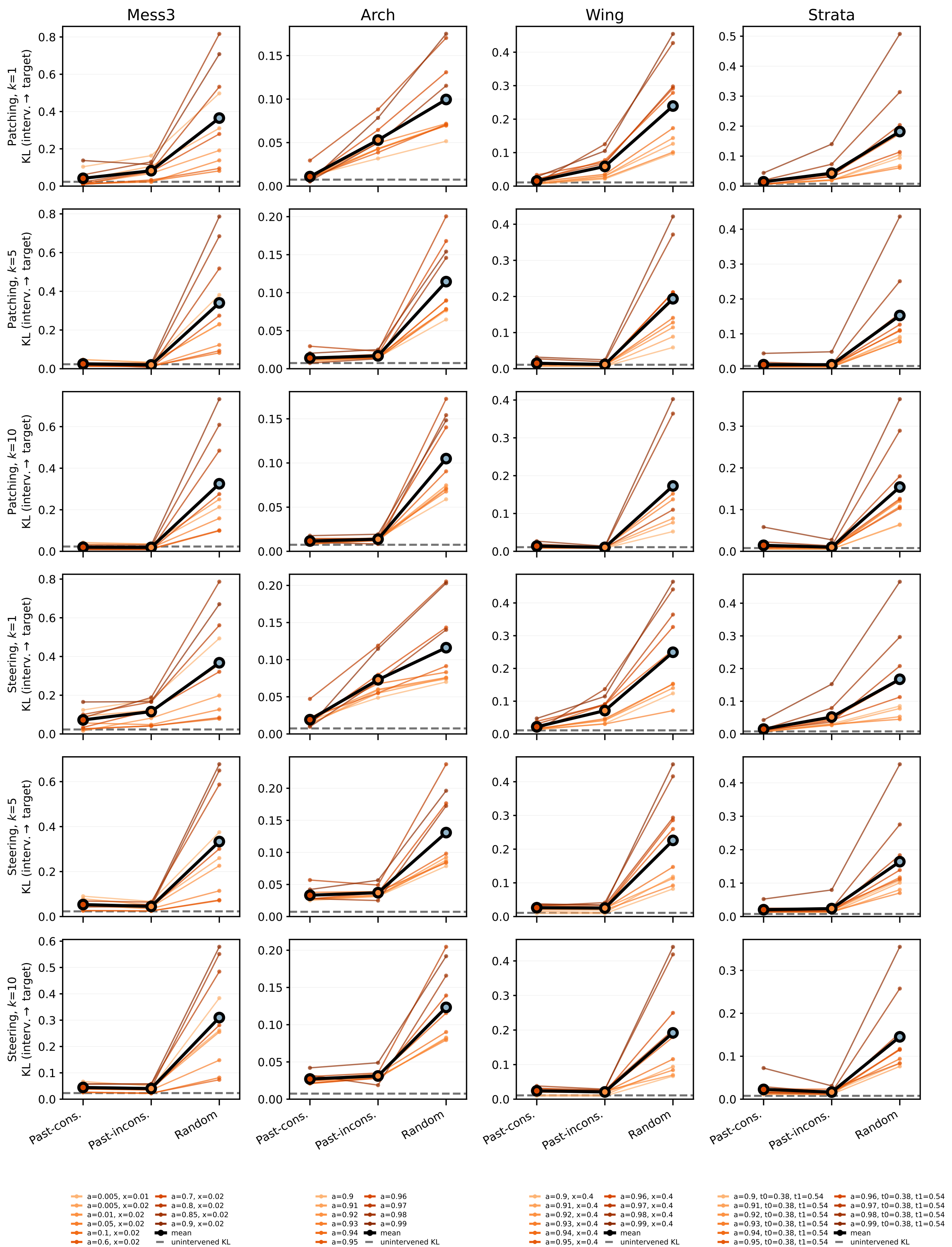
Qwen 3.5 9B (lower KL: prediction closer to injected target)
