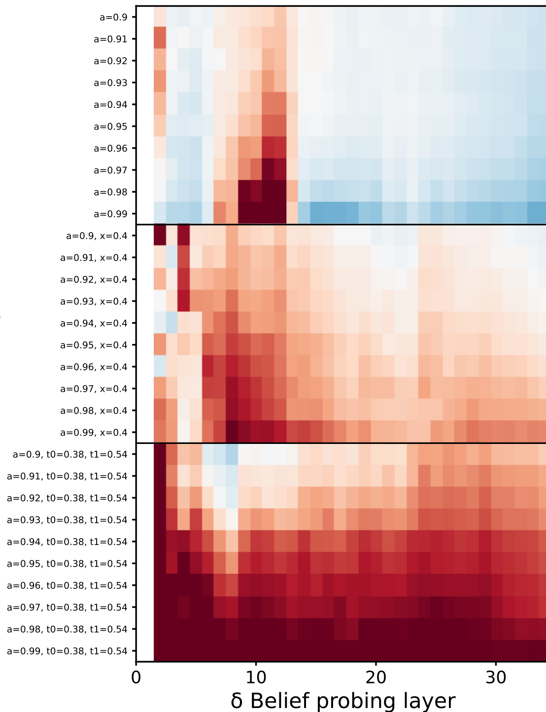
Target \delta -belief coordinate
