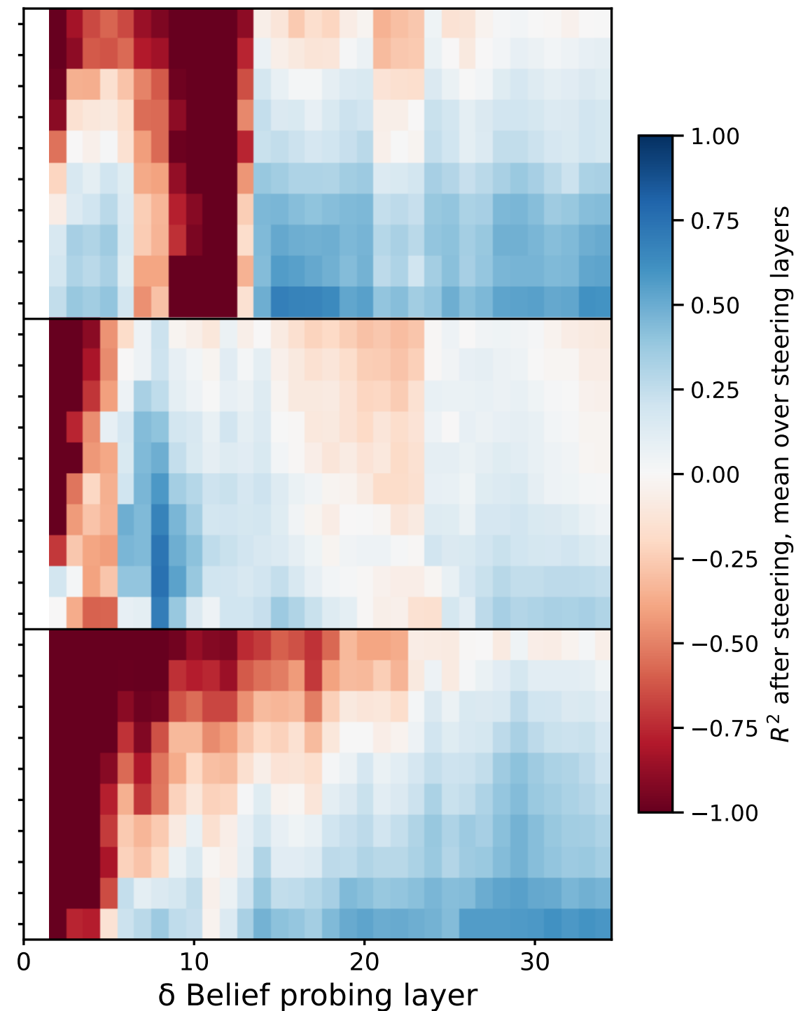
Original \delta -belief coordinate
