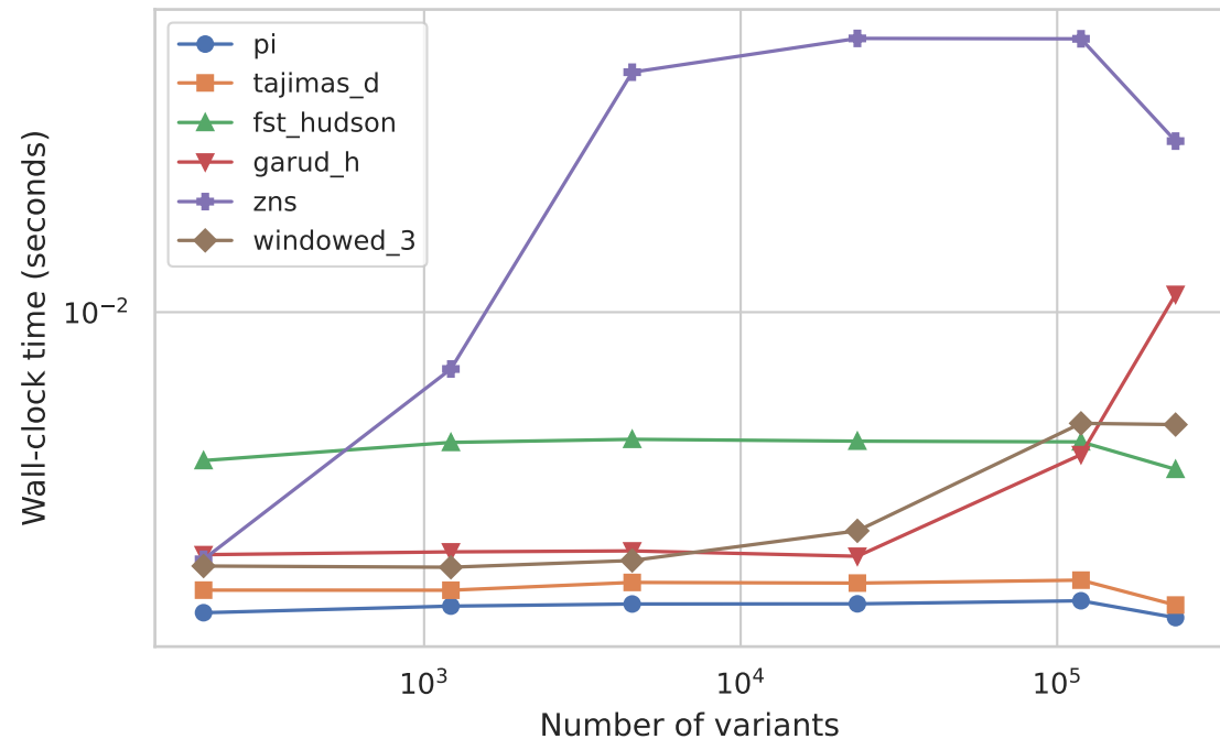
Runtime scaling with variant count (200 haplotypes)
