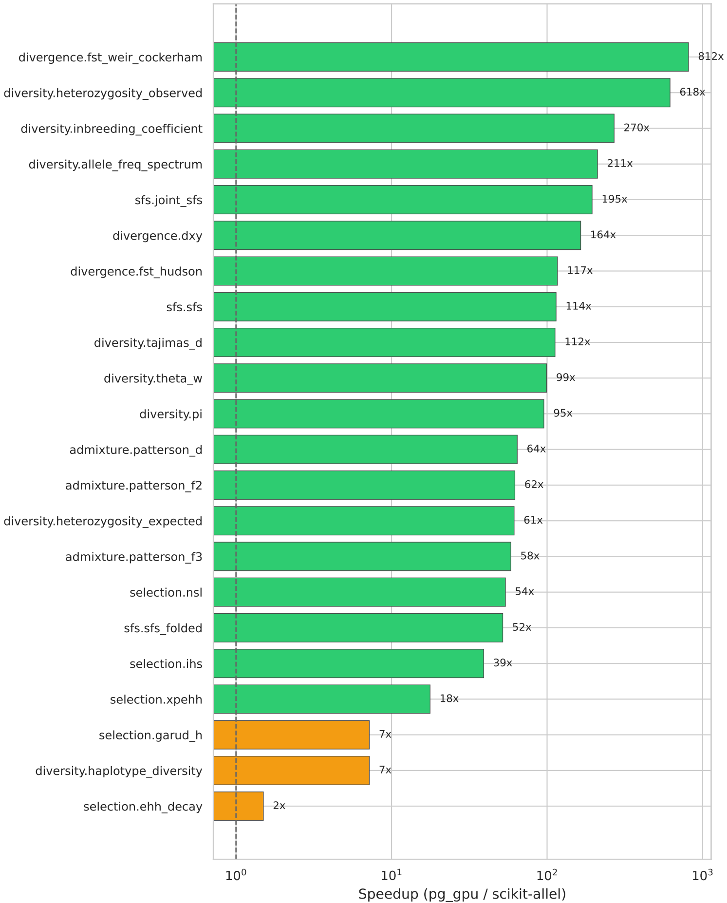
pg_gpu performance on Ag1000G 3R (2940 haplotypes, 10.9M variants)
