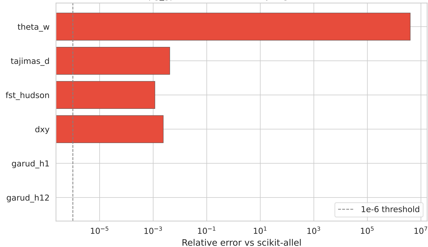
pg_gpu numerical accuracy (Ag1000G 3L)
