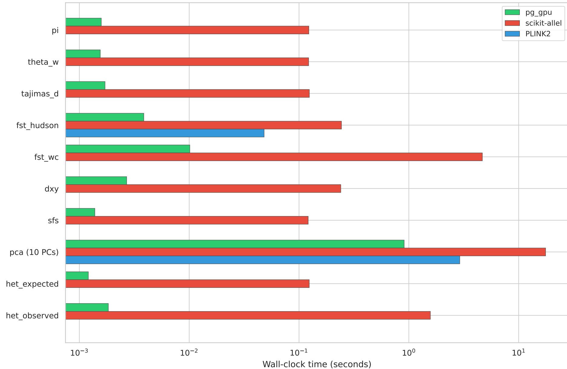
Performance: pg_gpu vs allele vs PLINK2 (2000 haplotypes, 45,685 variants, simulated)
