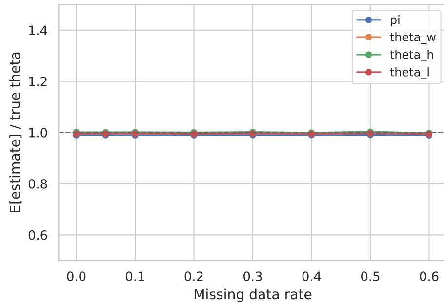
Theta estimator bias under MCAR
