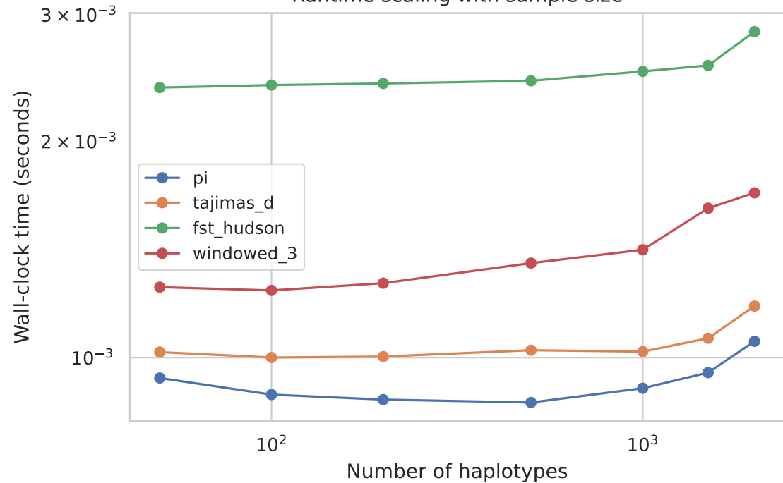
Runtime scaling with sample size
