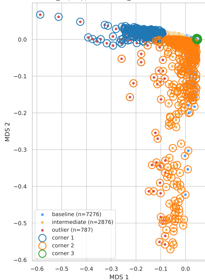
Local-PCA MDS along 3R (n_haplotypes=2940, n_windows=10939)
