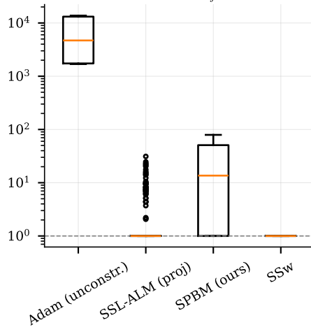
Feasibility Error \max_j (c_j - b)_+
