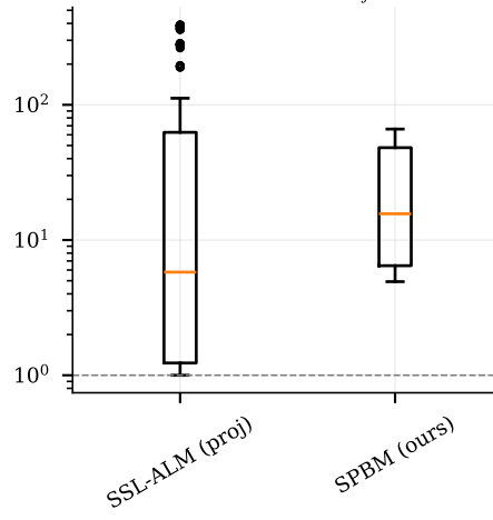
complementarity \sum_j |\lambda_j g_j|
