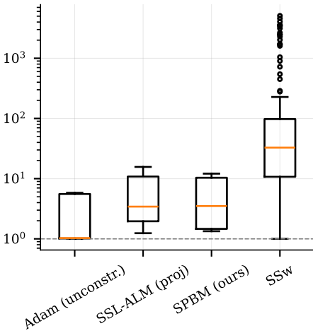
Stationarity Error, \|\nabla_x L\|
