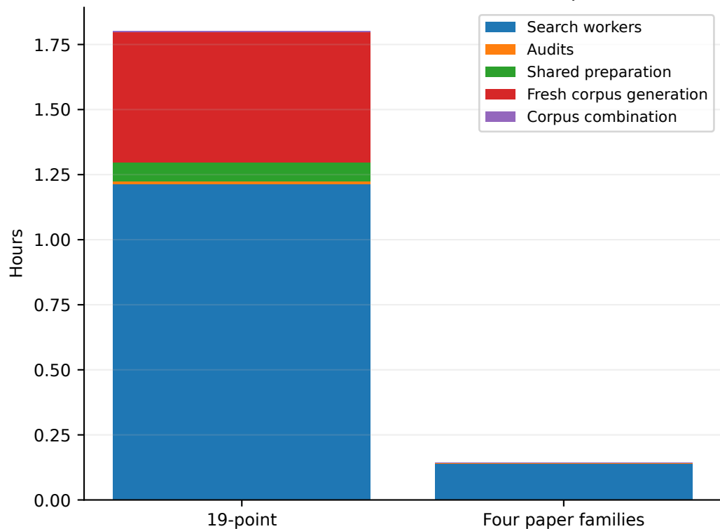
Summed recorded worker wall (not elapsed)
