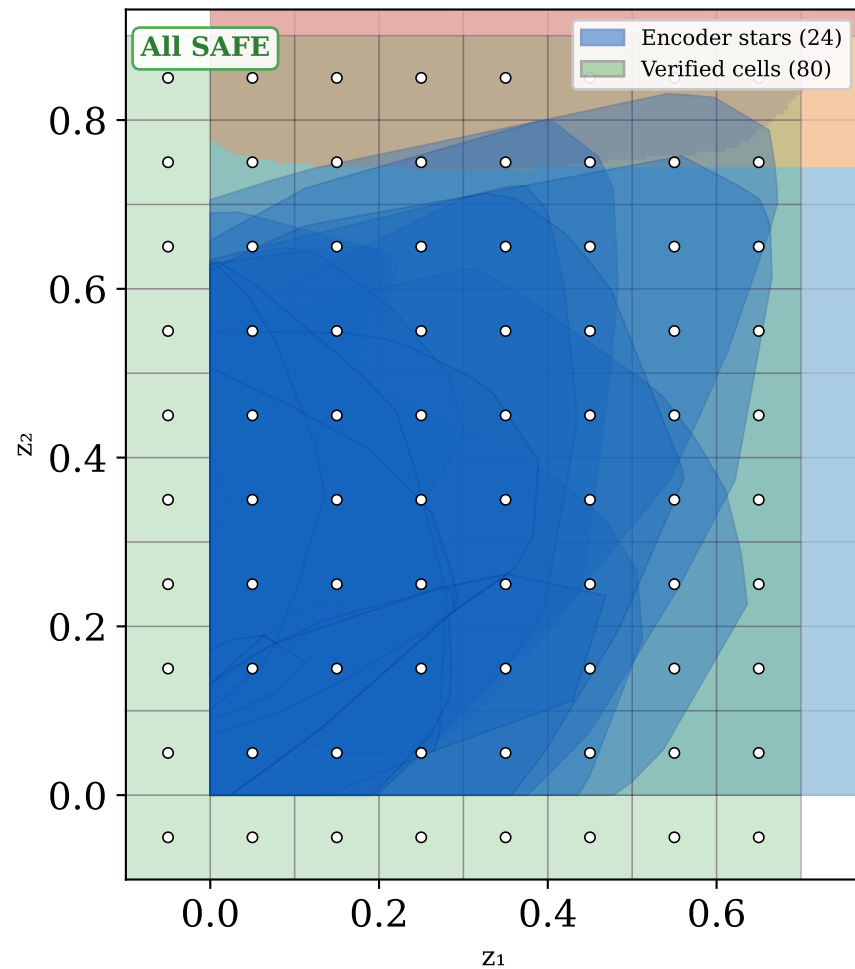
Encoder stars → quantized cells (spec 5)
