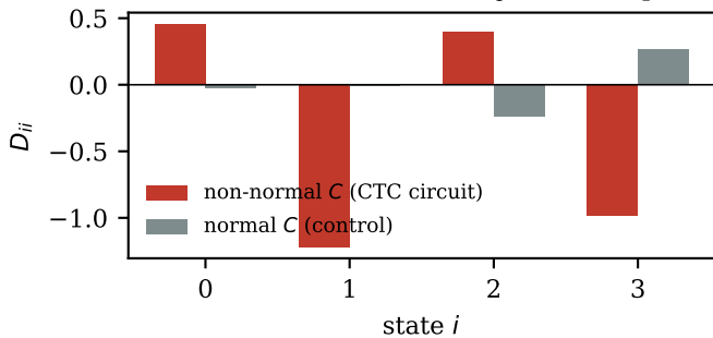
zero-work deviations, same job, same qubits
