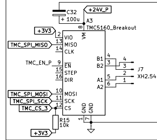
Joint Controller 6
