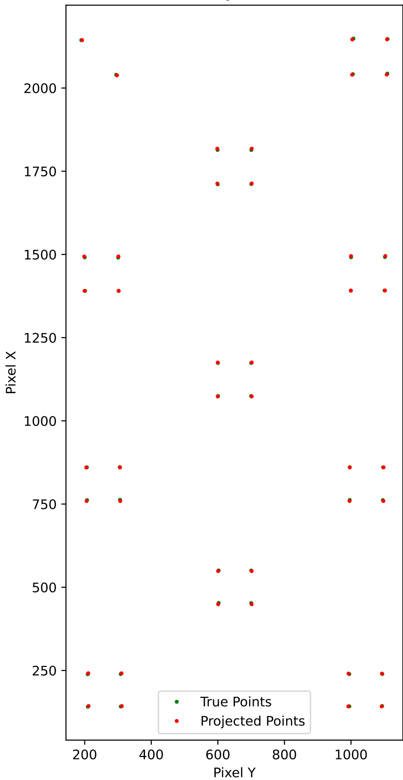
True vs Projected Points
