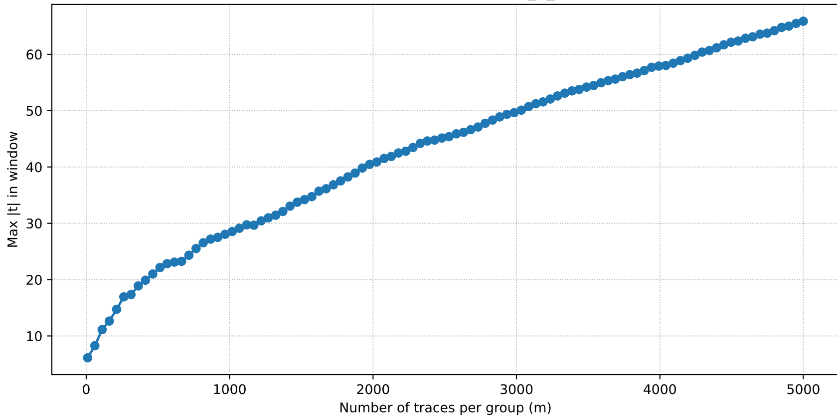
TVLA power curve — protected_4_neuron
