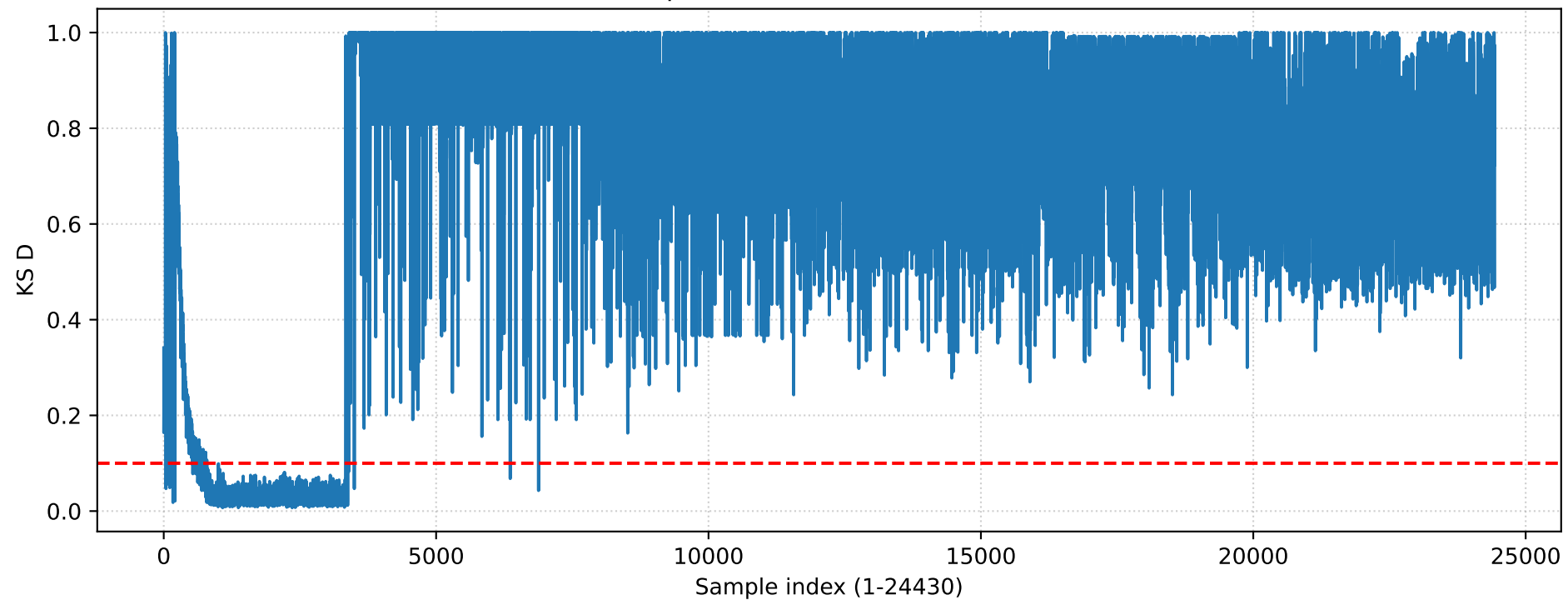
KSLA — unprotected7neuron (exceed=21708)
