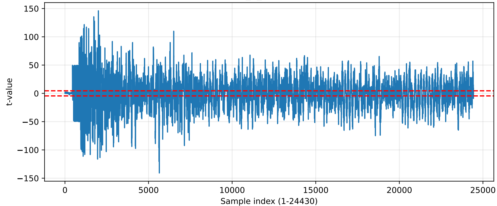
TVLA — protected_1_neuron (exceed=20489)
