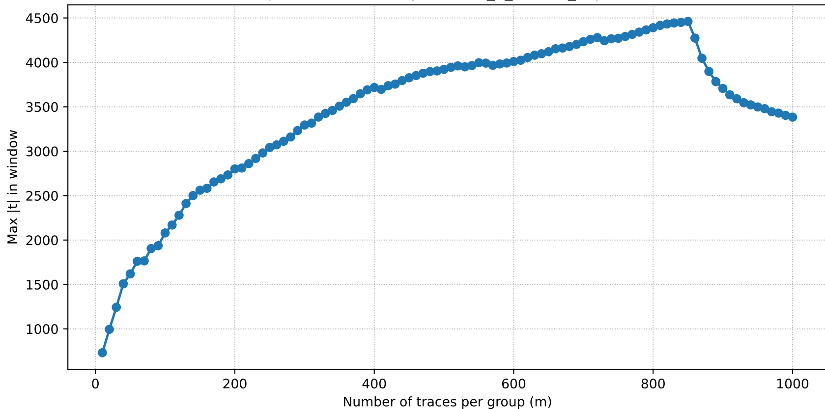
TVLA power curve — unprotected_7_neuron_exp(1-3000)
