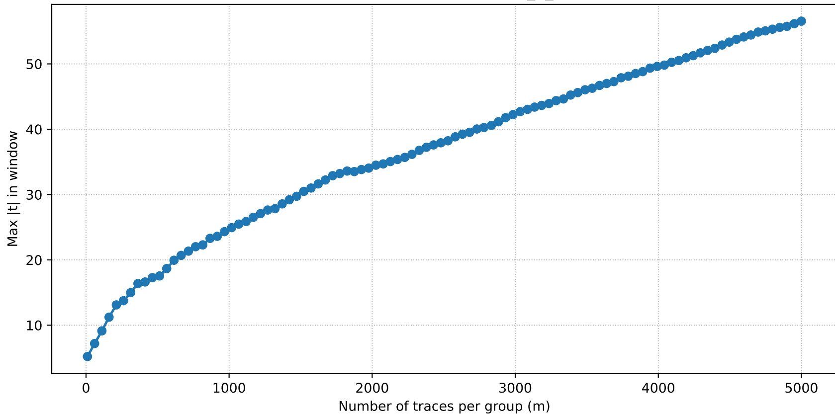
TVLA power curve — protected_1_neuron
