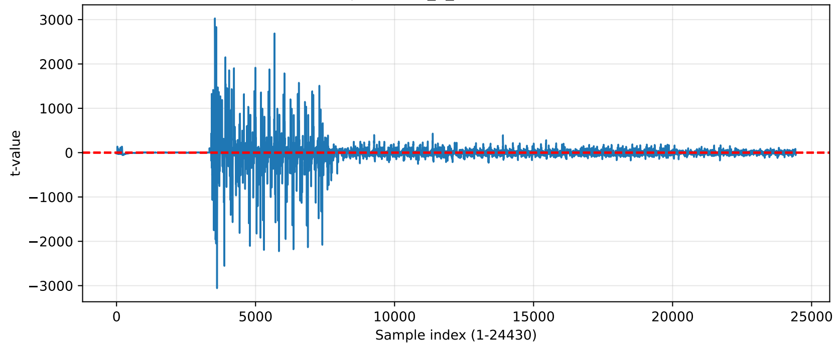
TVLA — unprotected_7_neuron (exceed=20309)
