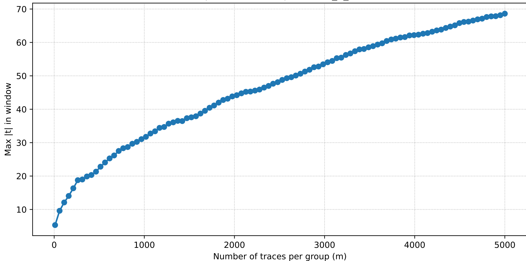
TVLA power curve — protected_6_neuron
