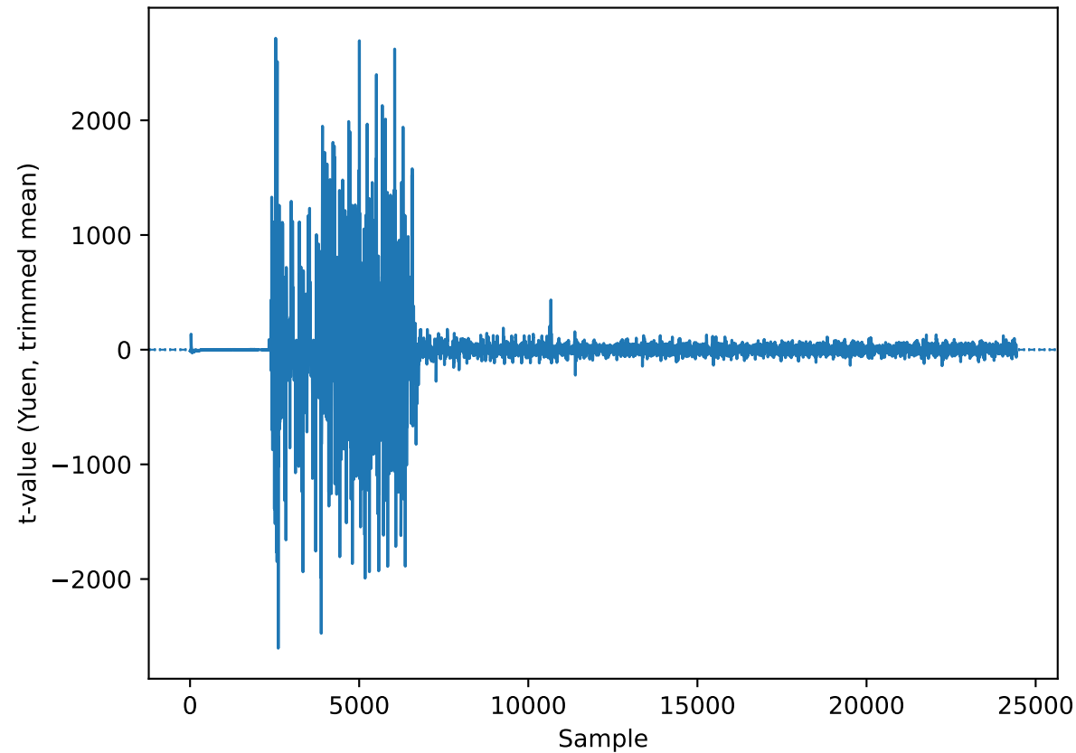
Yuen (trim=0.2) — unprotected5neuron (exceed=20312)
