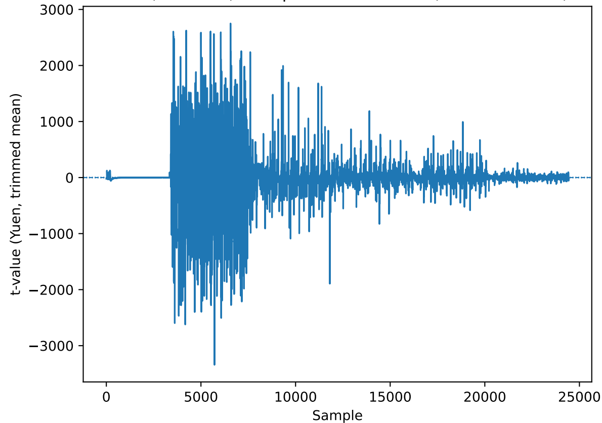
Yuen (trim=0.2) — unprotected7neuron (exceed=20384)
