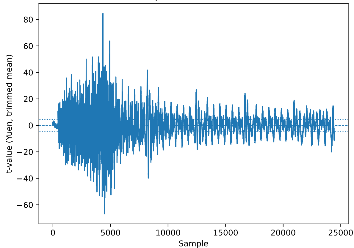
Yuen (trim=0.2) — protected2neuron (exceed=14485)
