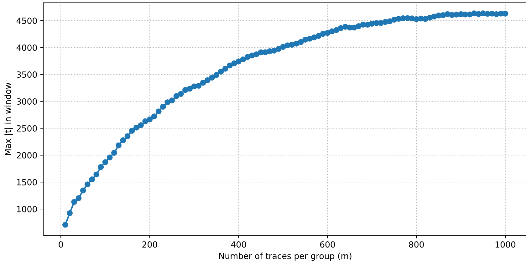
TVLA power curve — unprotected_6_neuron
