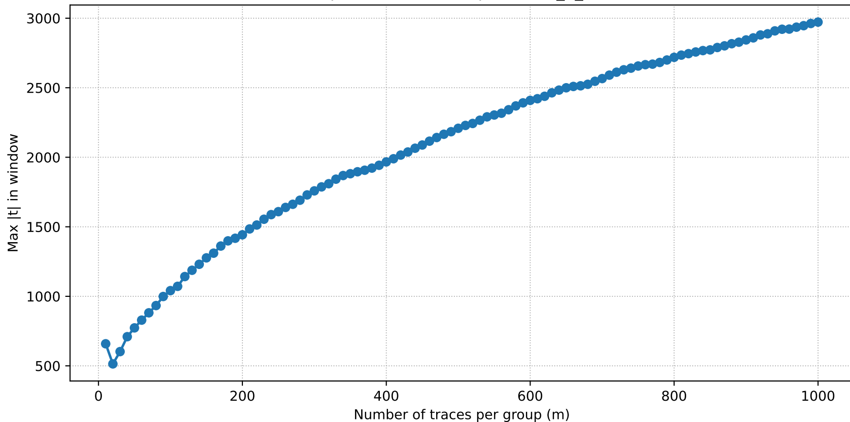
TVLA power curve — unprotected_5_neuron
