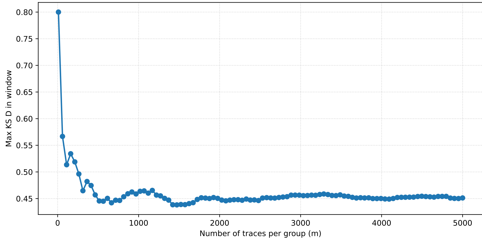
KSLA power curve — protected1neuron window=1000-4000, sliding L=512, step=256
