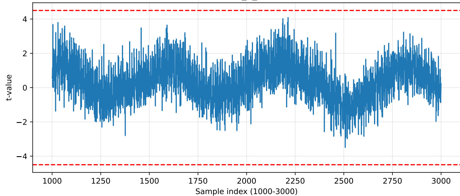
TVLA — unprotected_7_neuron (exceed=0)
