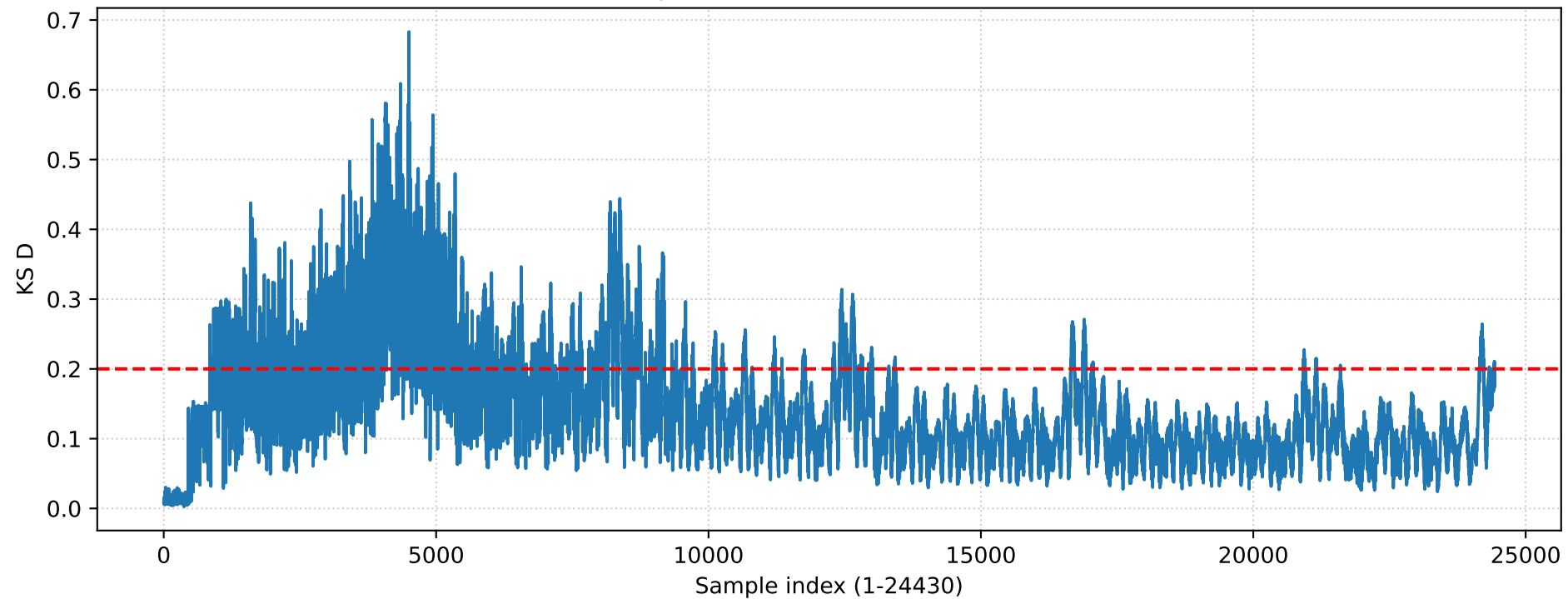
KSLA — protected7neuron (exceed=4695)
