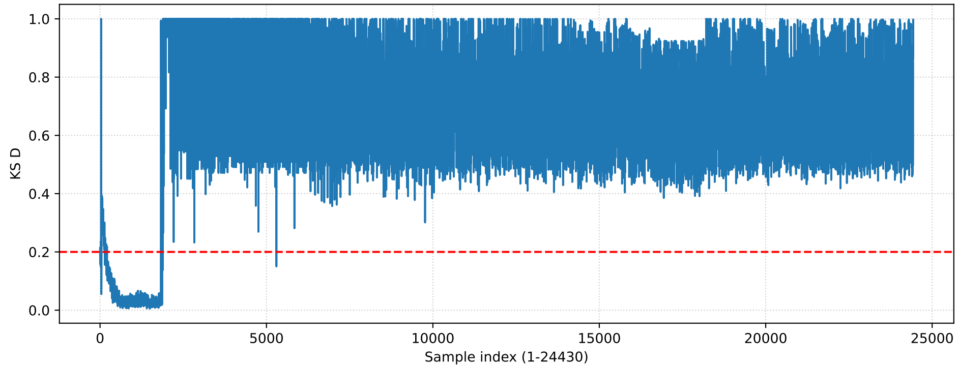
KSLA — unprotected4neuron (exceed=22710)
