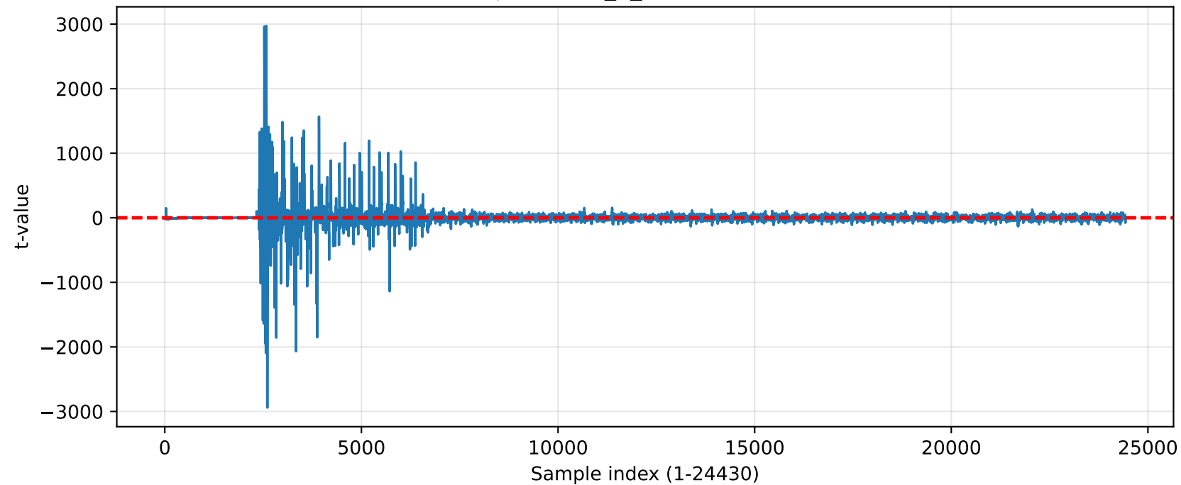
TVLA — unprotected_5_neuron (exceed=20554)
