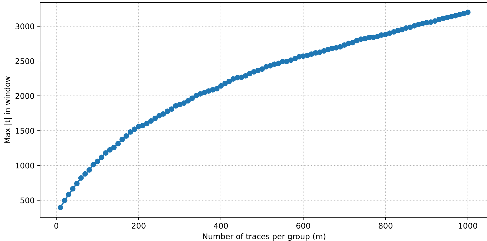
TVLA power curve — unprotected_4_neuron
