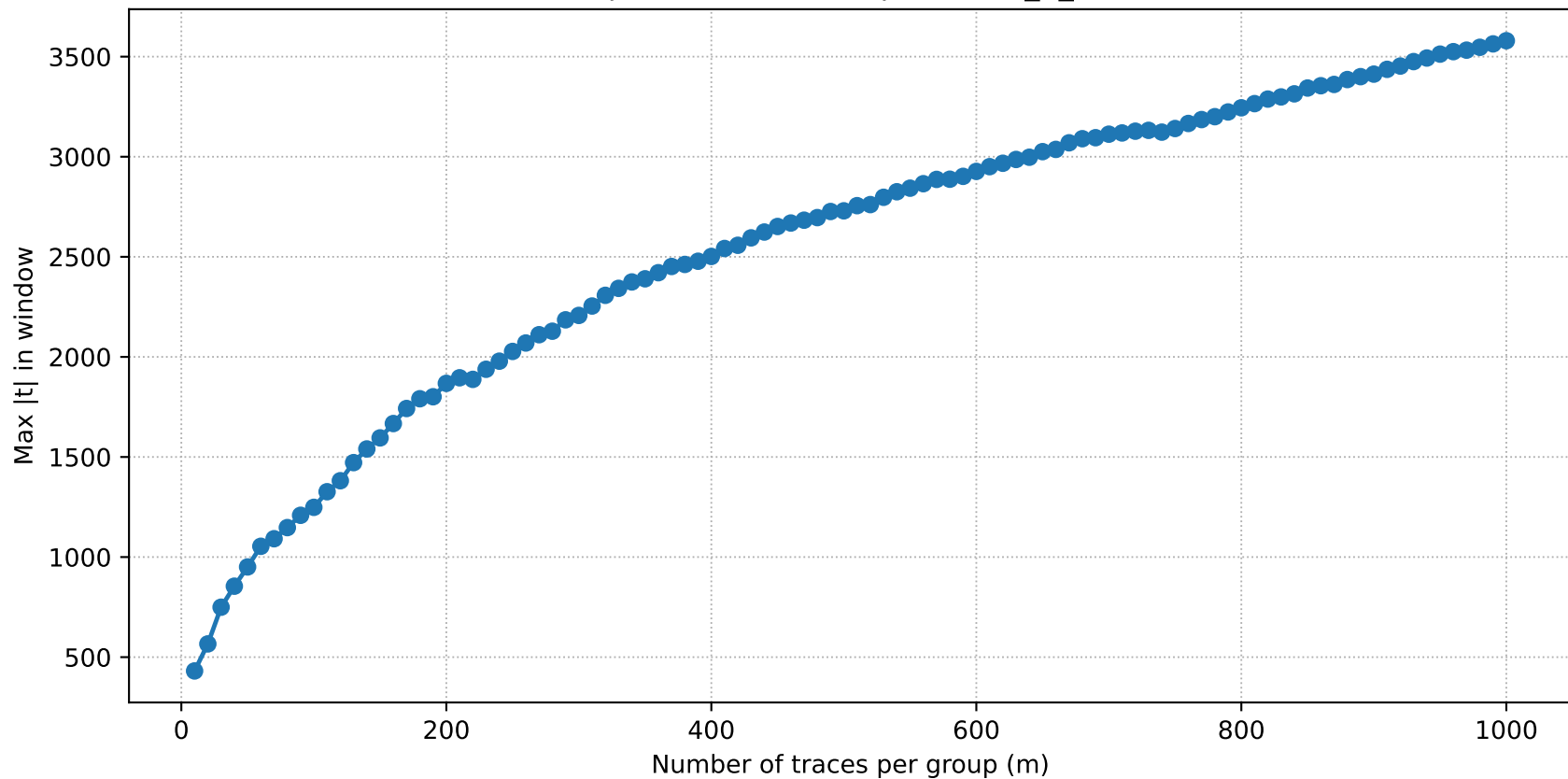
TVLA power curve — unprotected_3_neuron
