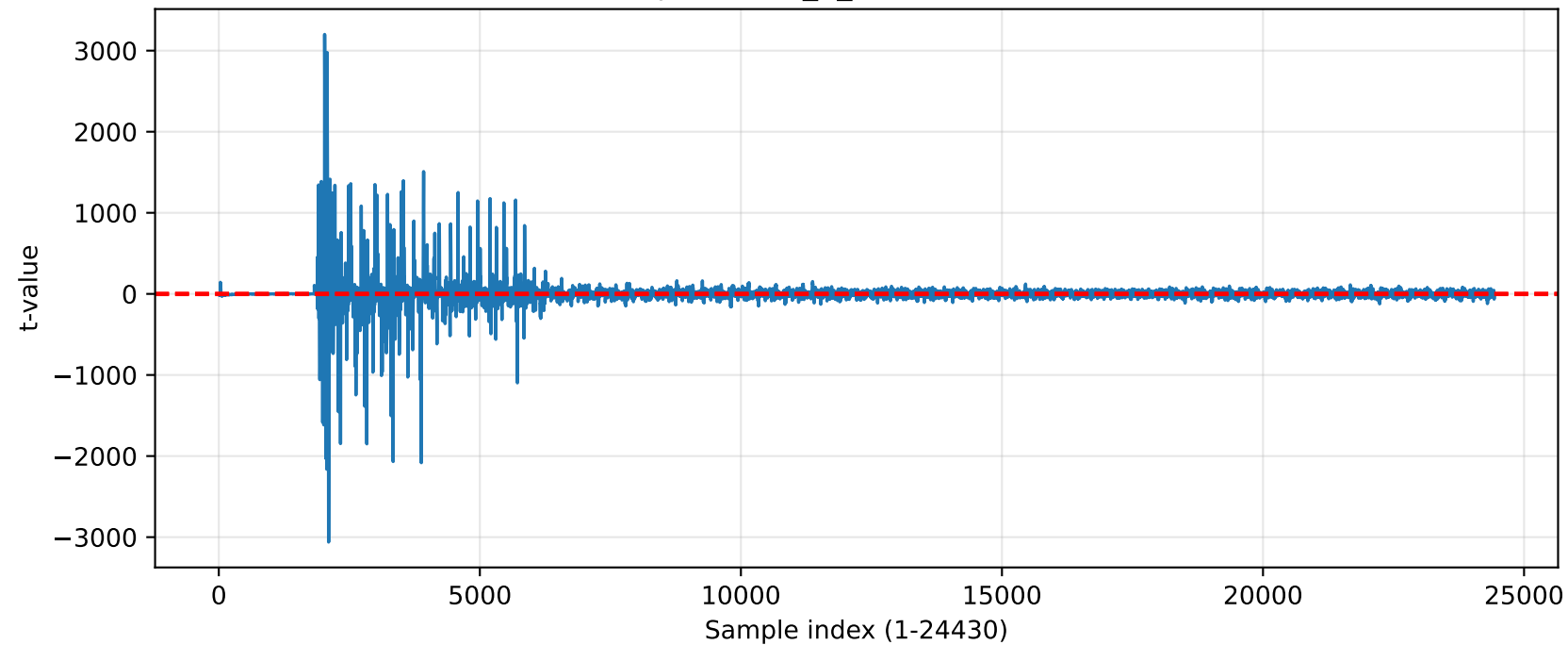
TVLA — unprotected_4_neuron (exceed=20984)
