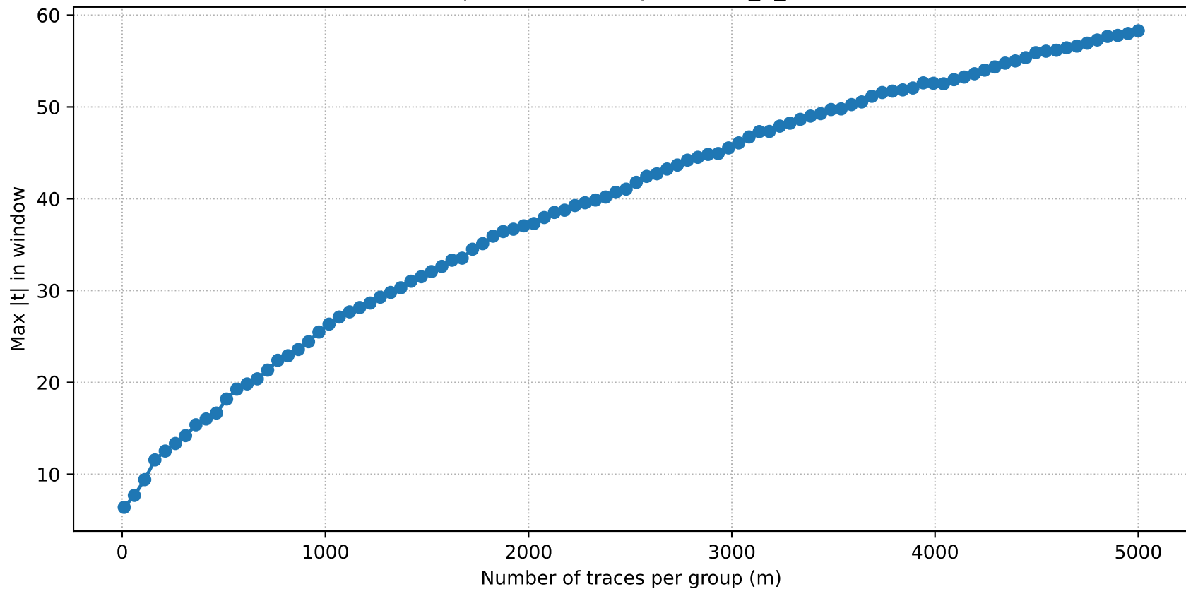
TVLA power curve — protected_2_neuron
