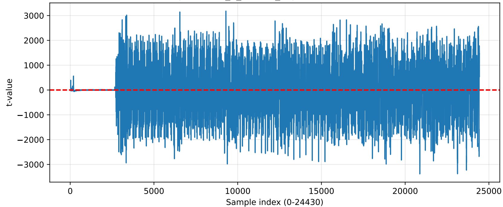
TVLA — unprotected_7_neuron_exp(1-3000) (exceed=24062)
