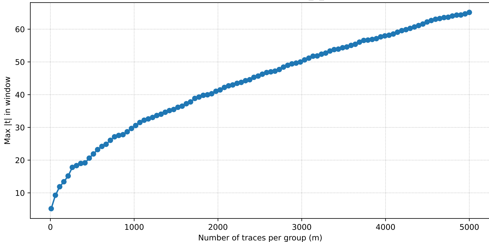
TVLA power curve — protected_5_neuron
