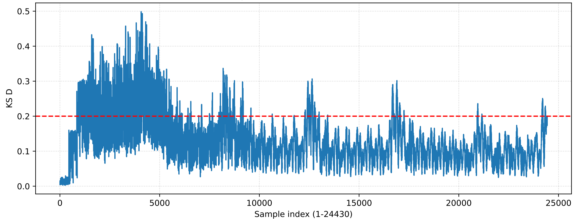
KSLA — protected3neuron (exceed=3523)
