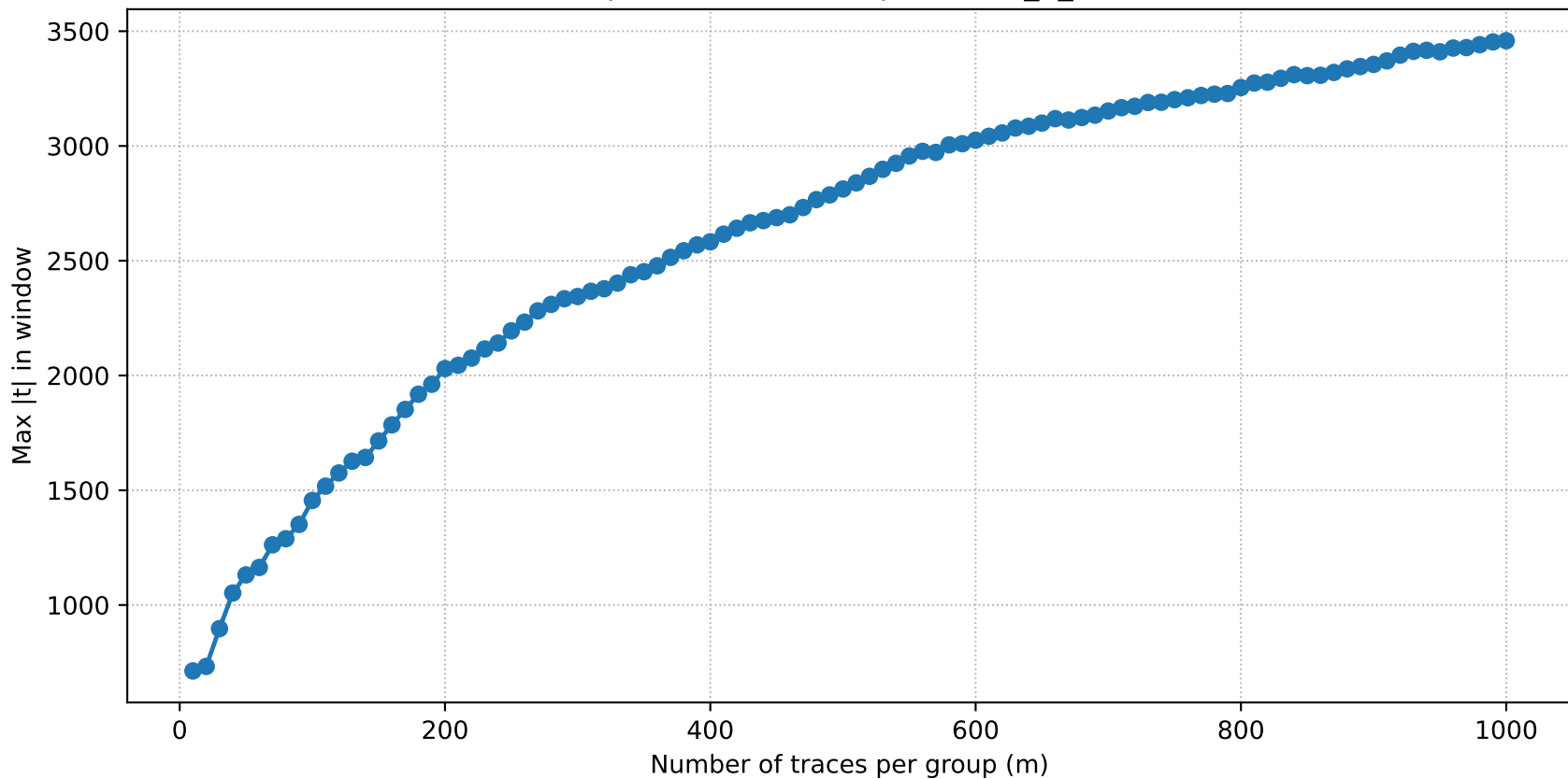
TVLA power curve — unprotected_1_neuron
