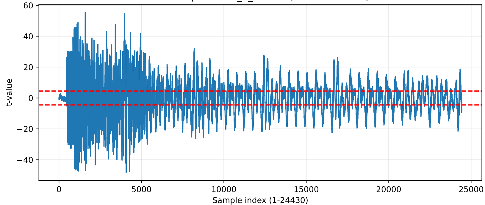
TVLA — protected_3_neuron (exceed=15722)
