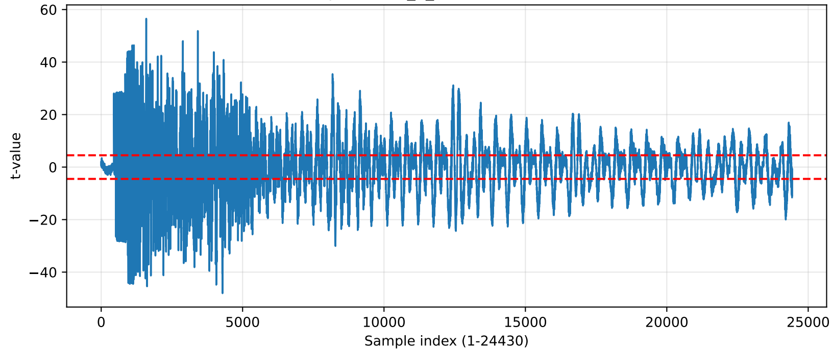
TVLA — protected_1_neuron (exceed=15389)
