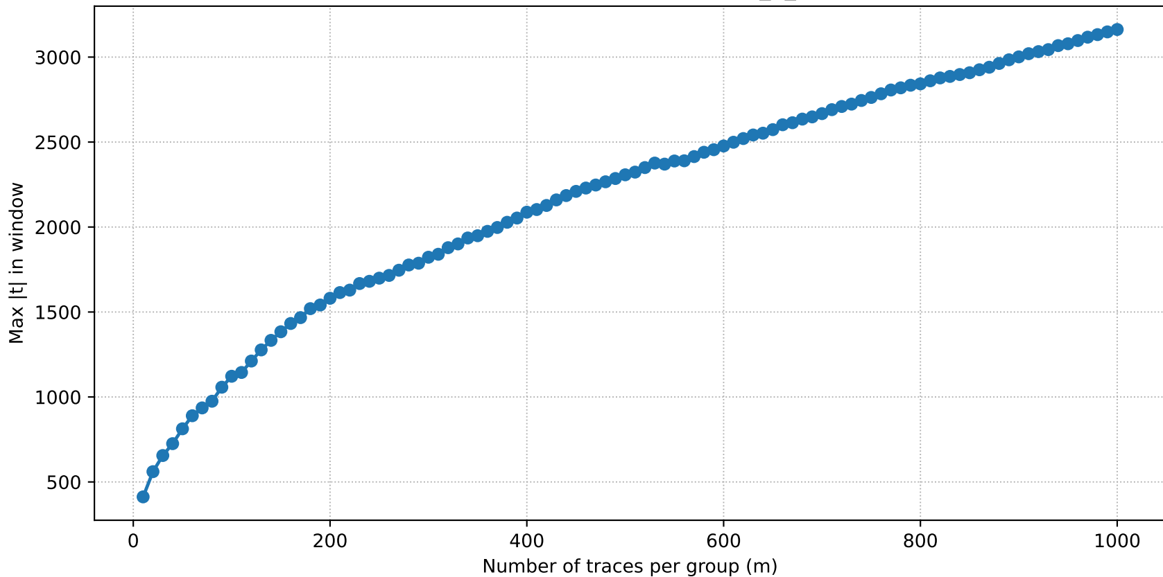
TVLA power curve — unprotected_2_neuron
