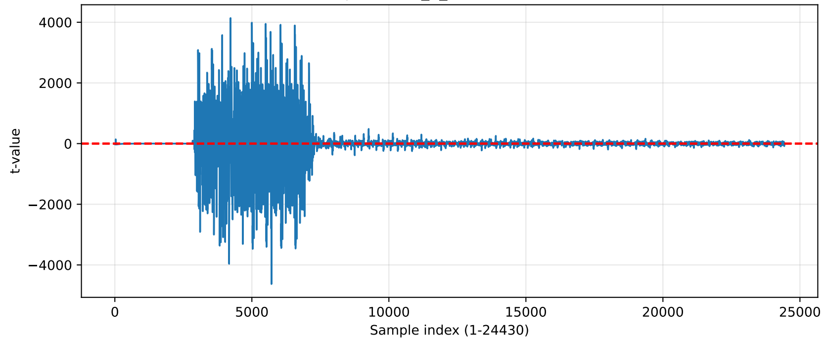
TVLA — unprotected_6_neuron (exceed=20464)
