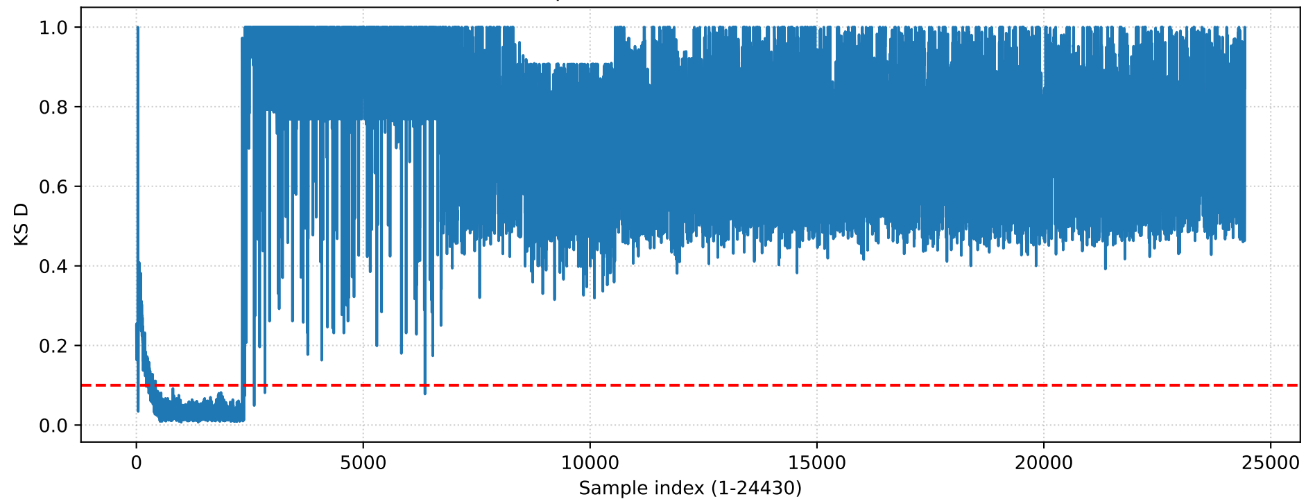
KSLA — unprotected5neuron (exceed=22397)
