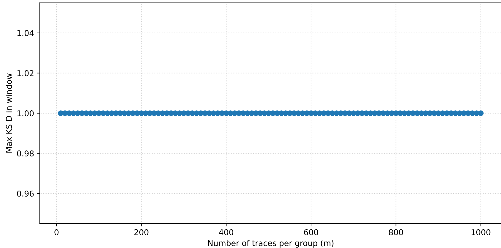
KSLA power curve — unprotected7neuron window=1000-4000, sliding L=512, step=256
