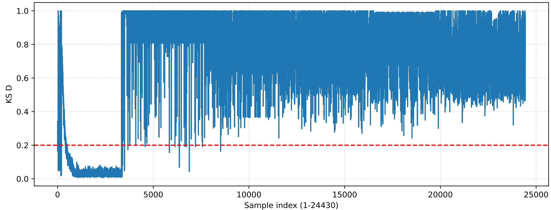
KSLA — unprotected7neuron (exceed=21471)
