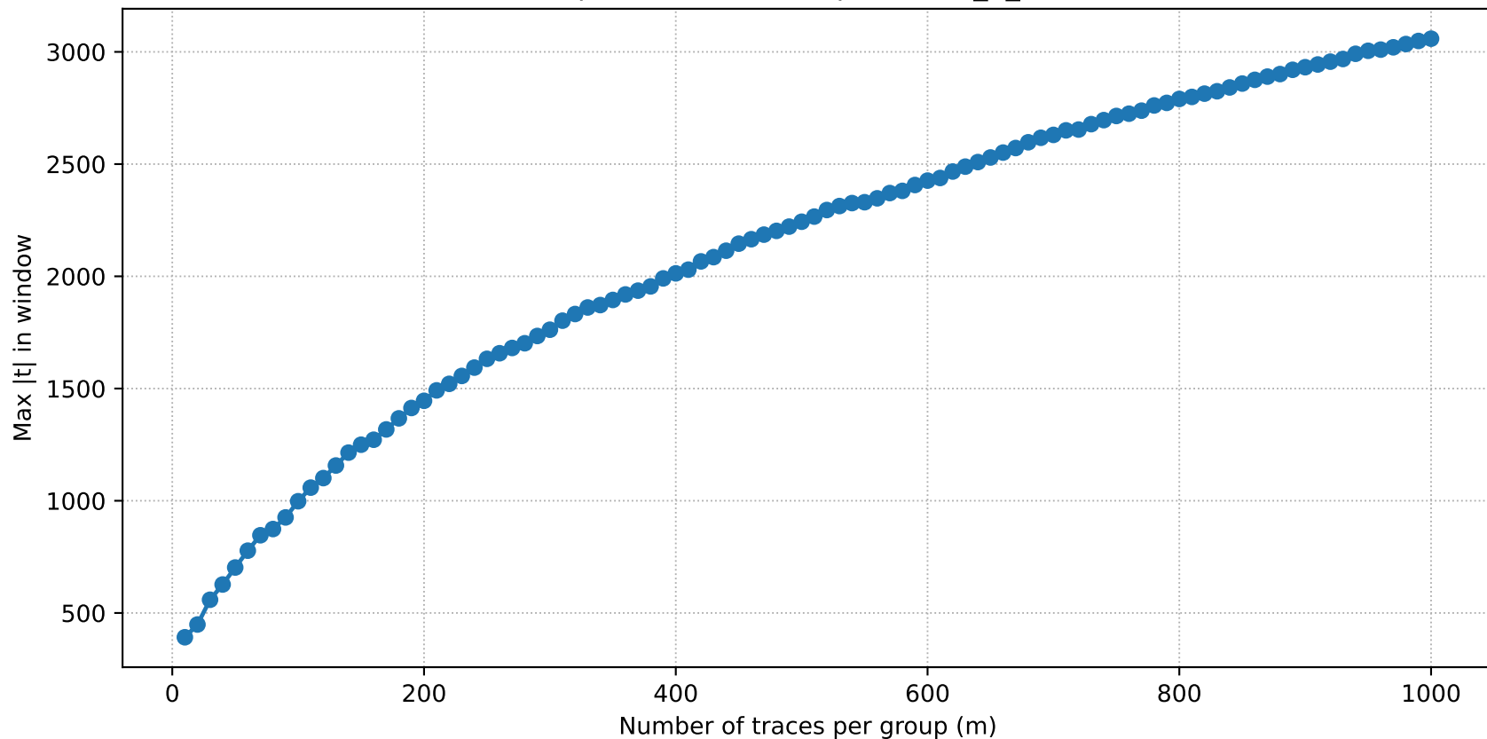
TVLA power curve — unprotected_7_neuron
