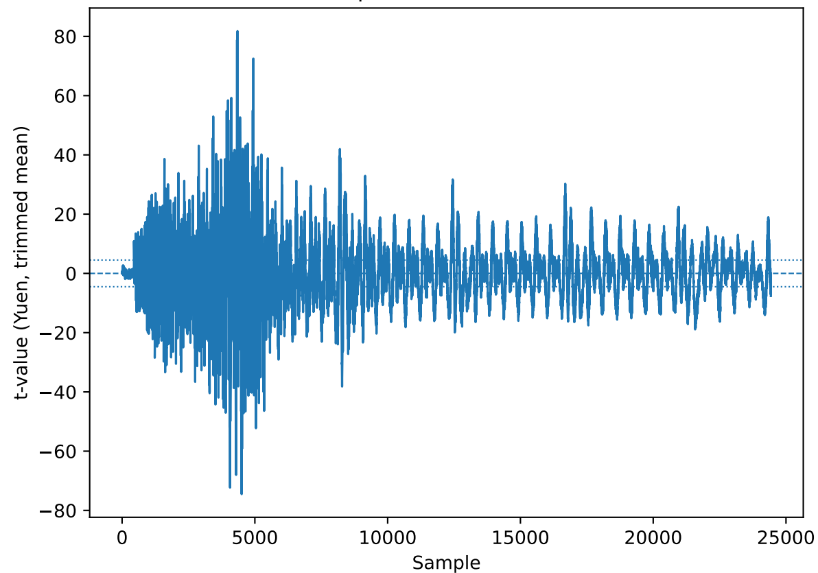
Yuen (trim=0.2) — protected5neuron (exceed=15093)
