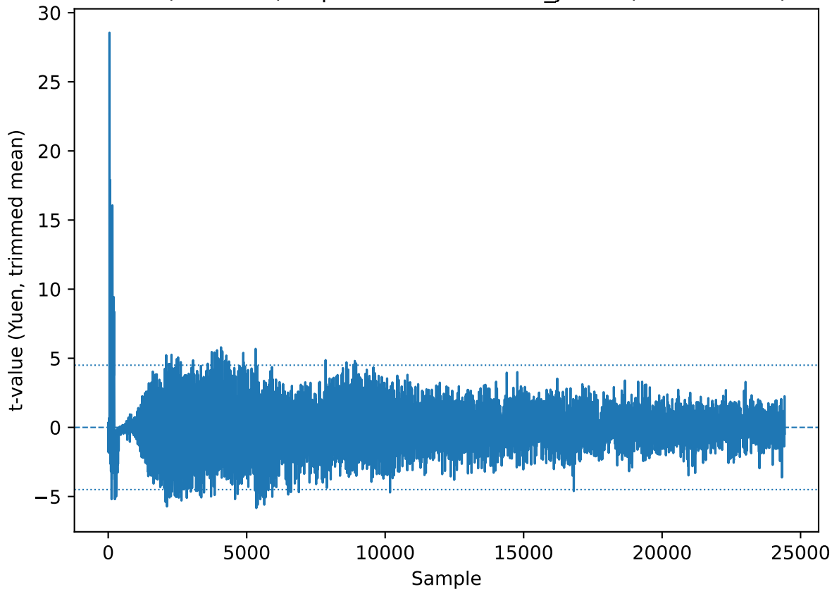
Yuen (trim=0.2) — protected1stneuron_jitters (exceed=227)
