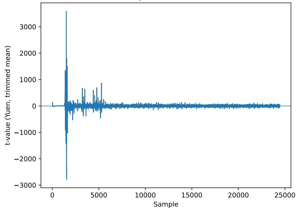
Yuen (trim=0.2) — unprotected3neuron (exceed=20908)
