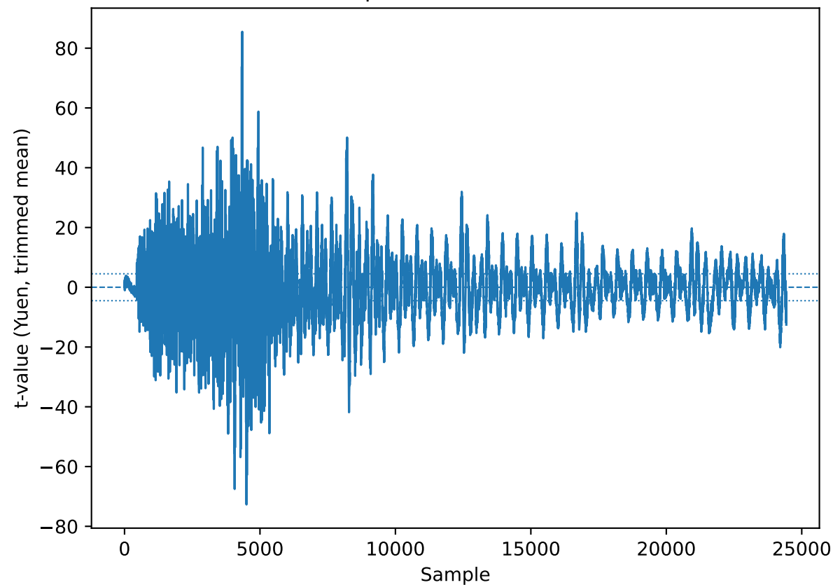
Yuen (trim=0.2) — protected4neuron (exceed=14881)
