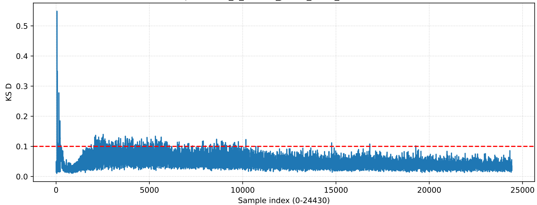
KSLA — protected_1_neuron_jitters_KSLA_0.1 (exceed=511)
