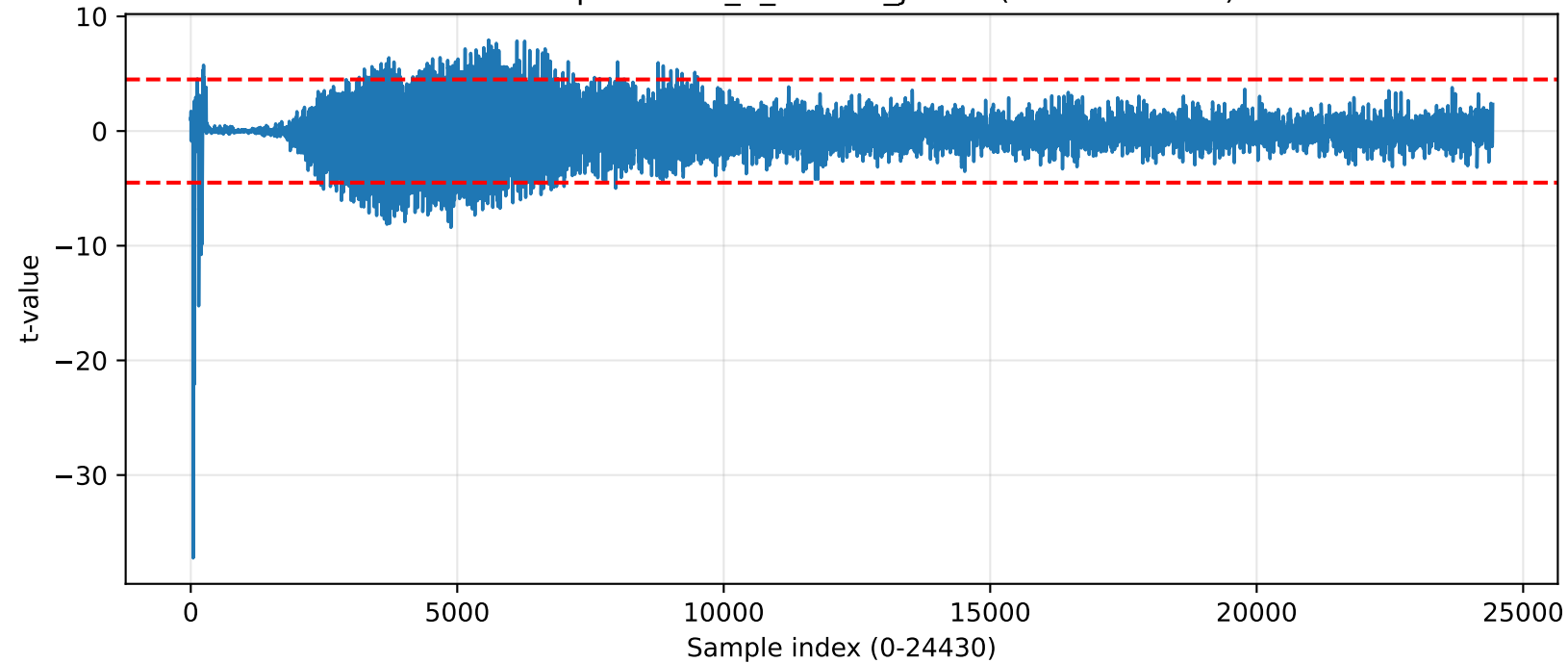
TVLA — protected_1_neuron_jitters (exceed=1036)
