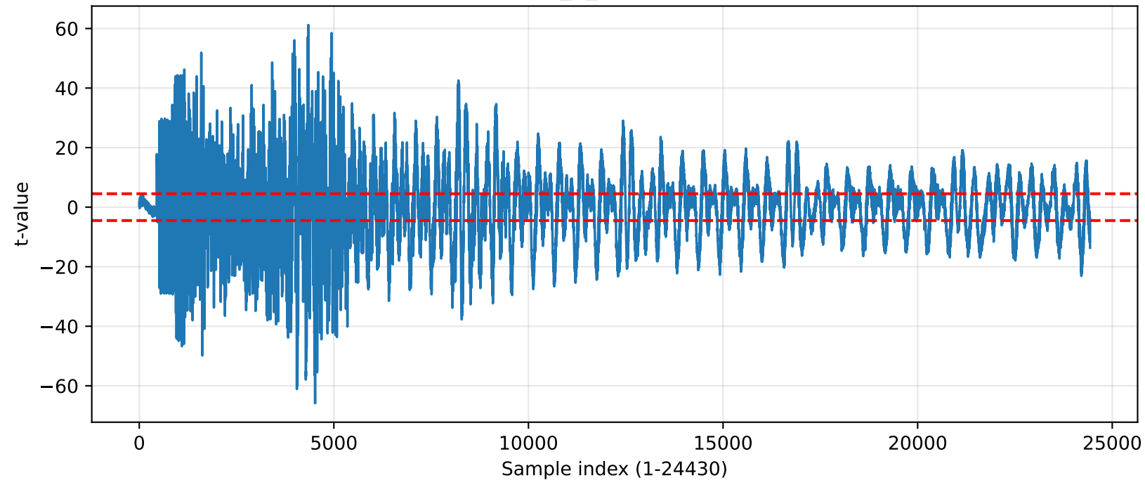
TVLA — protected_4_neuron (exceed=16206)
