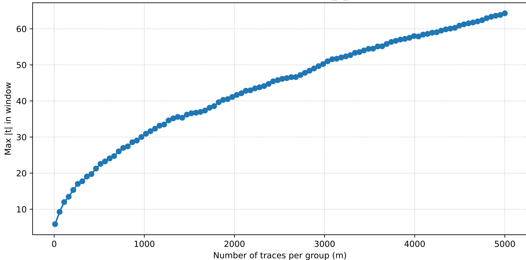
TVLA power curve — protected_7_neuron
