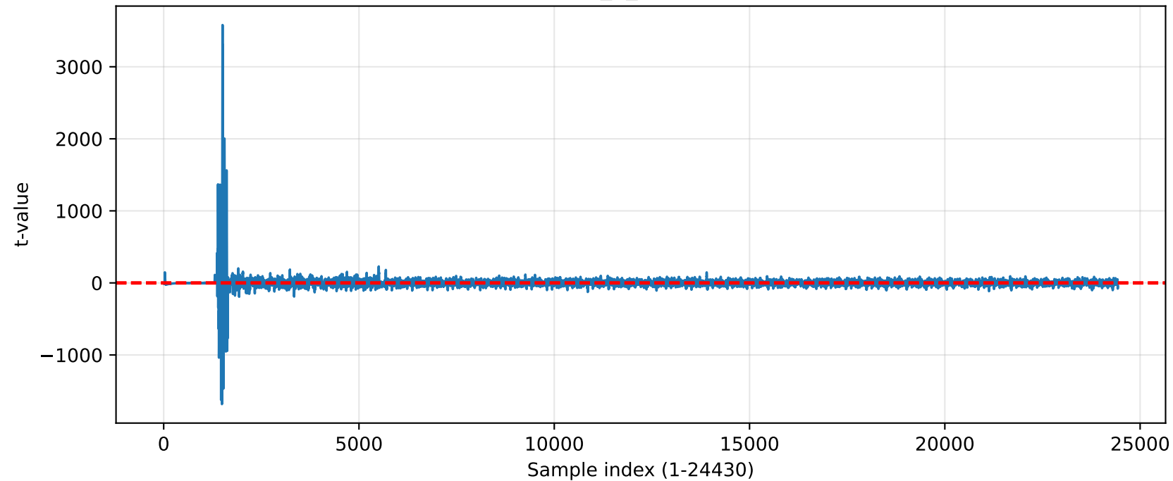
TVLA — unprotected_3_neuron (exceed=21353)
