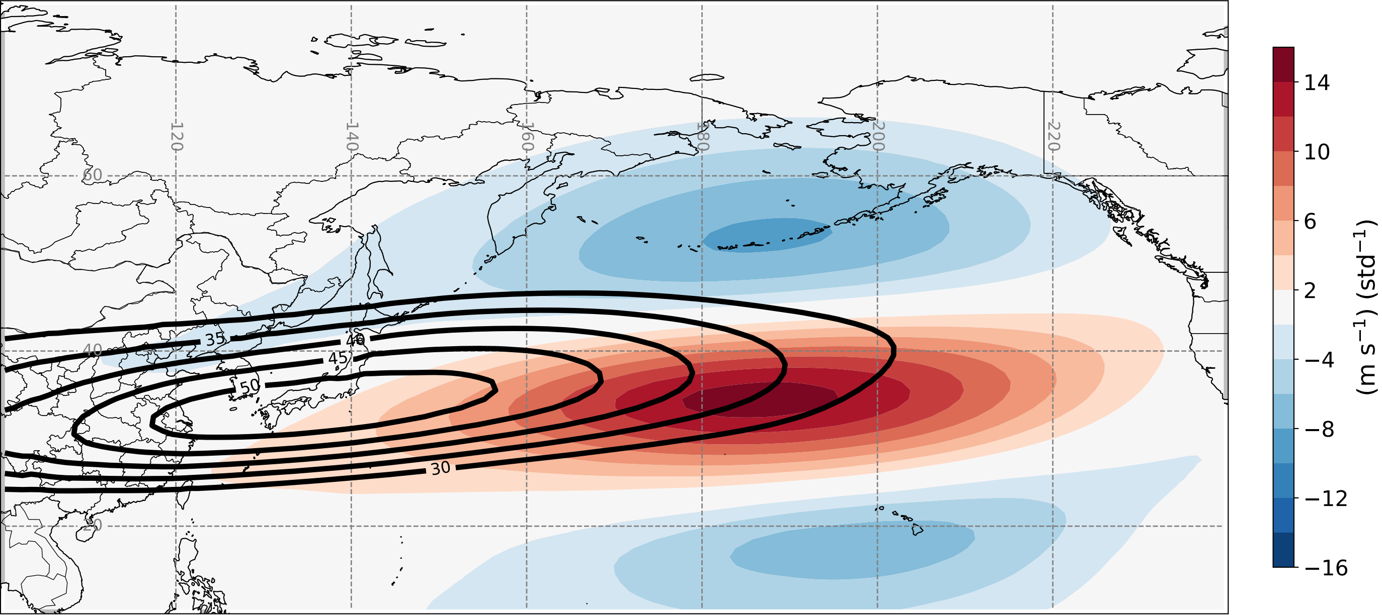
ERA5 EOF1 of 200-hPa Zonal Wind Anomalies (Sept-May 1979-2014)
