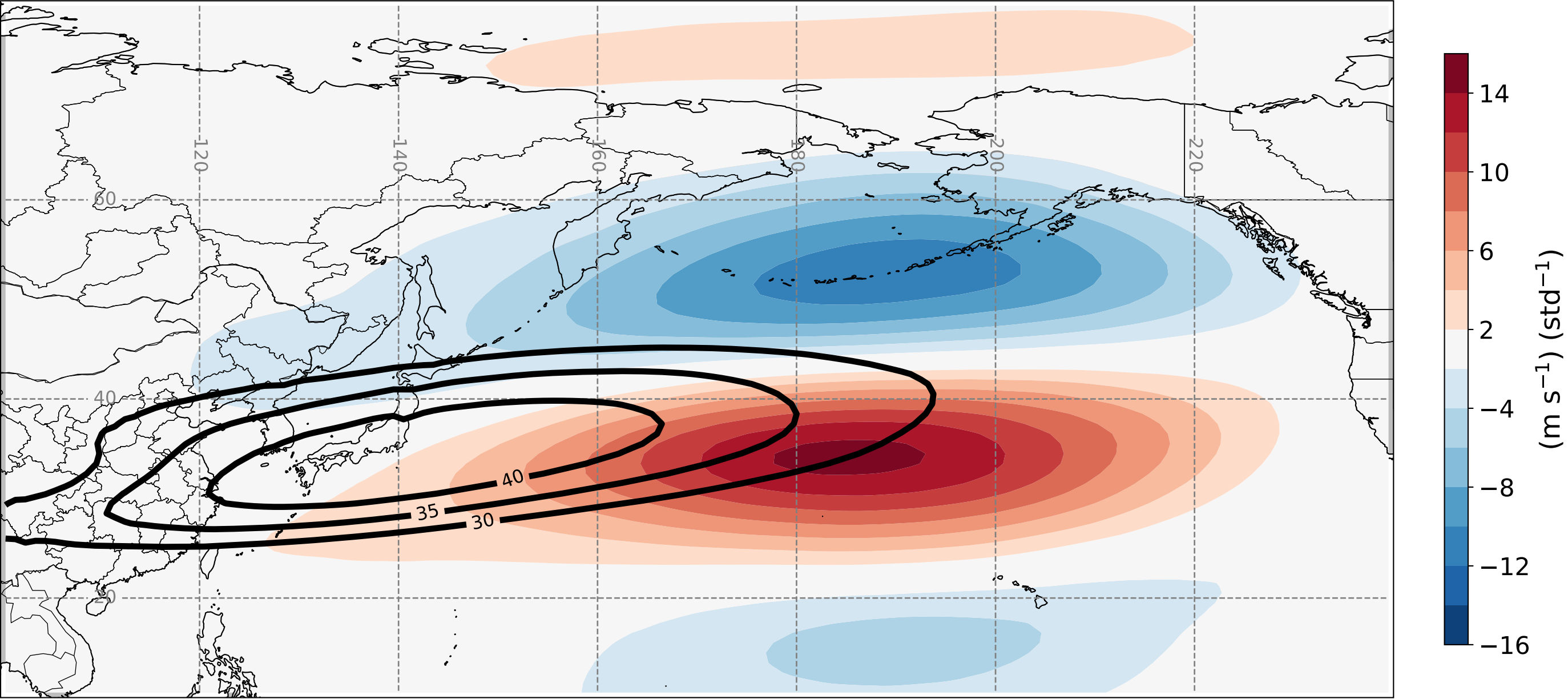
ERA5 EOF1 of 300-hPa Zonal Wind Anomalies (Sept-May 1979-2014)
