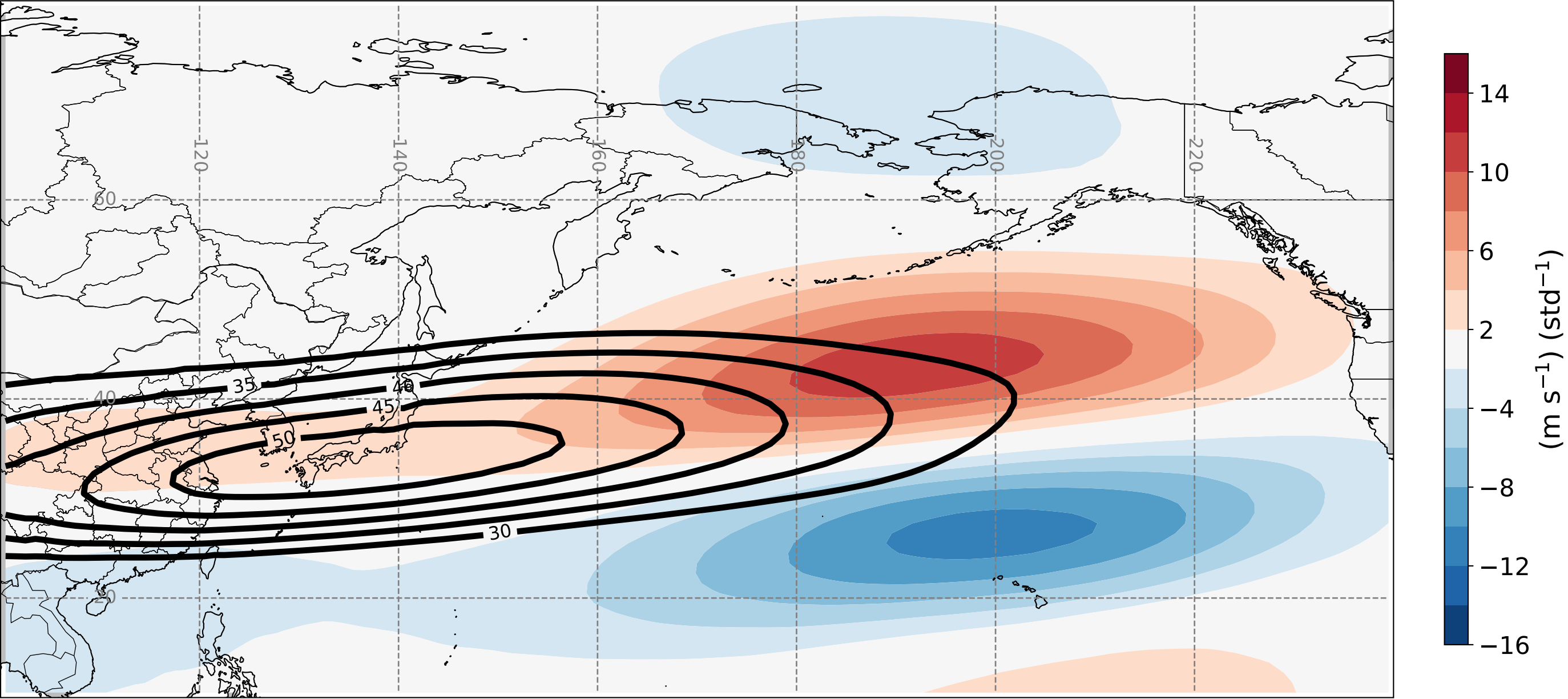
ERA5 EOF2 of 200-hPa Zonal Wind Anomalies (Sept-May 1979-2014)
