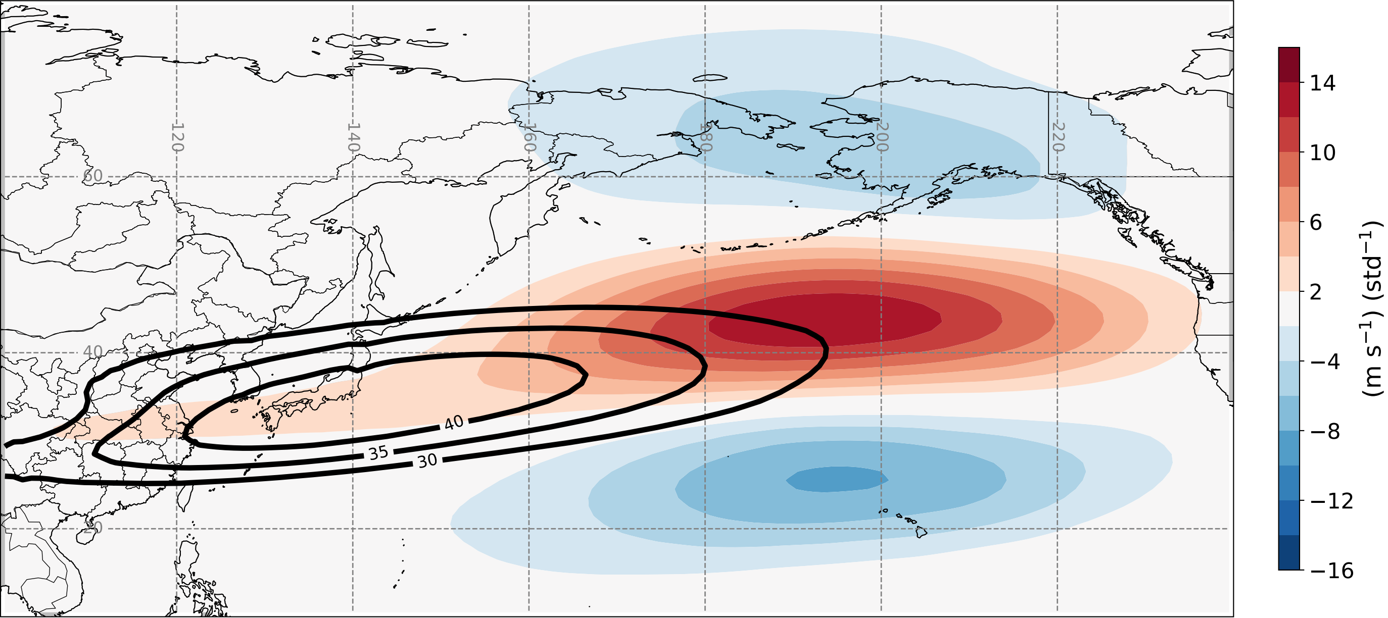
ERA5 EOF2 of 300-hPa Zonal Wind Anomalies (Sept-May 1979-2014)
