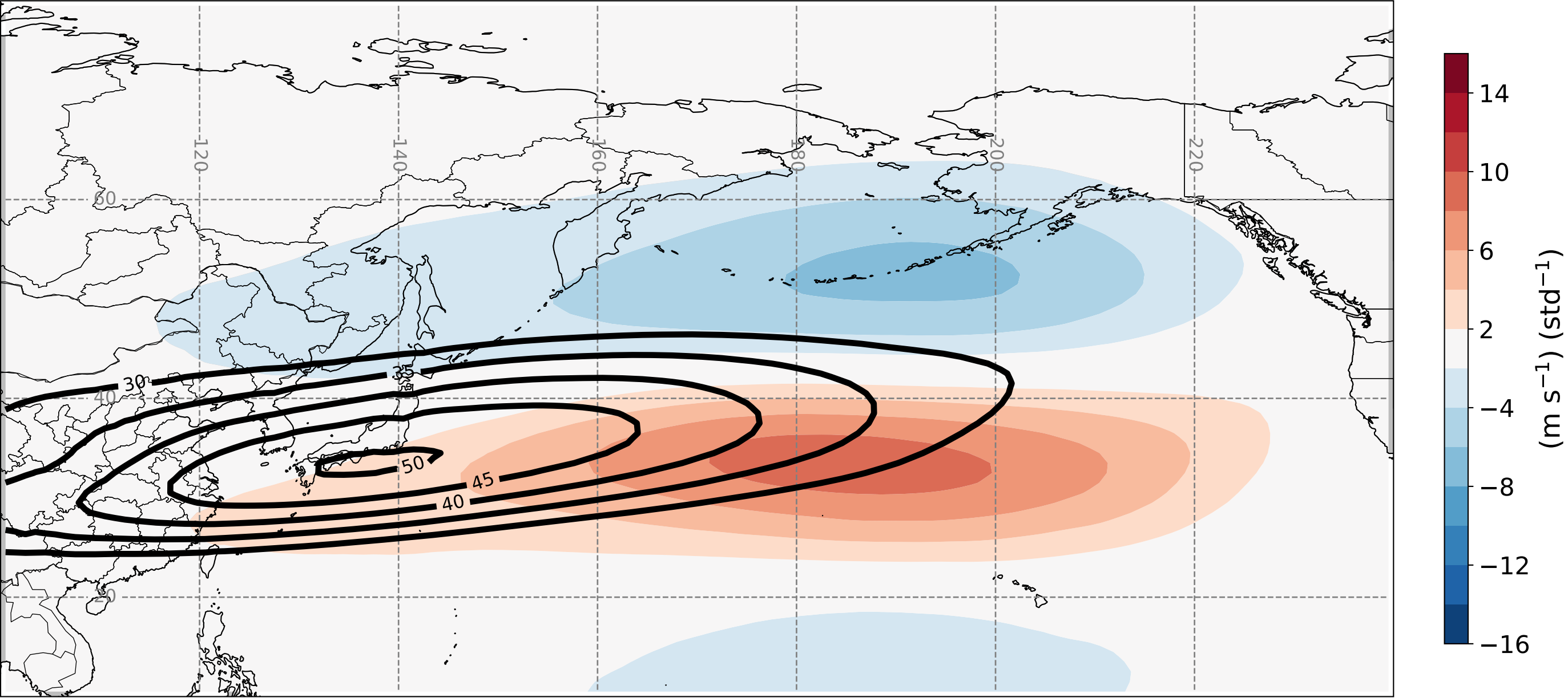
ERA5 EOF1 of 250-hPa Zonal Wind Anomalies (Sept-May 1979-2014)
