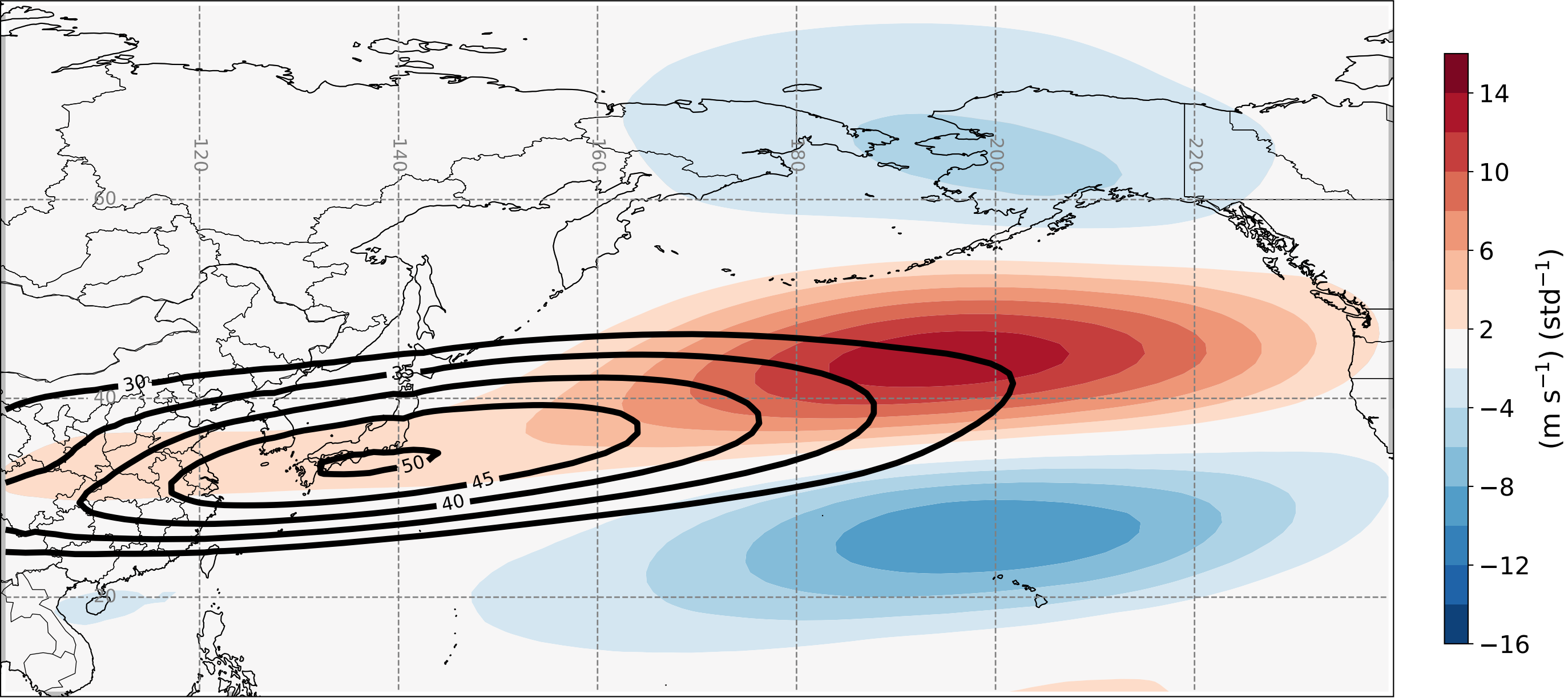
ERA5 EOF2 of 250-hPa Zonal Wind Anomalies (Sept-May 1979-2014)
