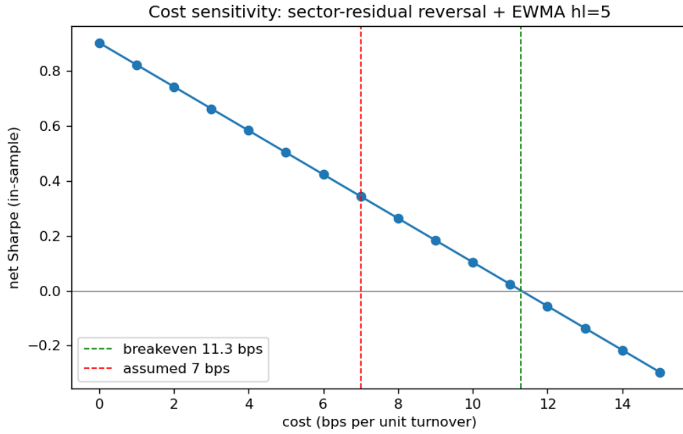
Figure 1: In-sample net Sharpe versus assumed per-turnover cost. Net-positive up to the \sim 11.3 bps break-even; about 0.08 Sharpe lost per bp.
